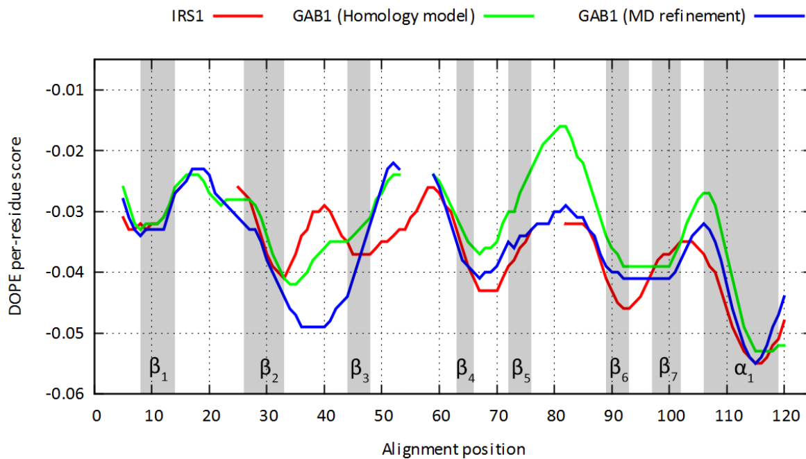
Figure S4. Comparison of DOPE score profiles. IRS1 (PDB ID: 1QQG), GAB1 homology model and the lowest energy GAB1 model with MD simulation refinement were compared. The MD refinement model was subject to 1000 steps energy minimization with ff99SB force field to remove transient structural defects. The secondary structure is annotated at the bottom.
