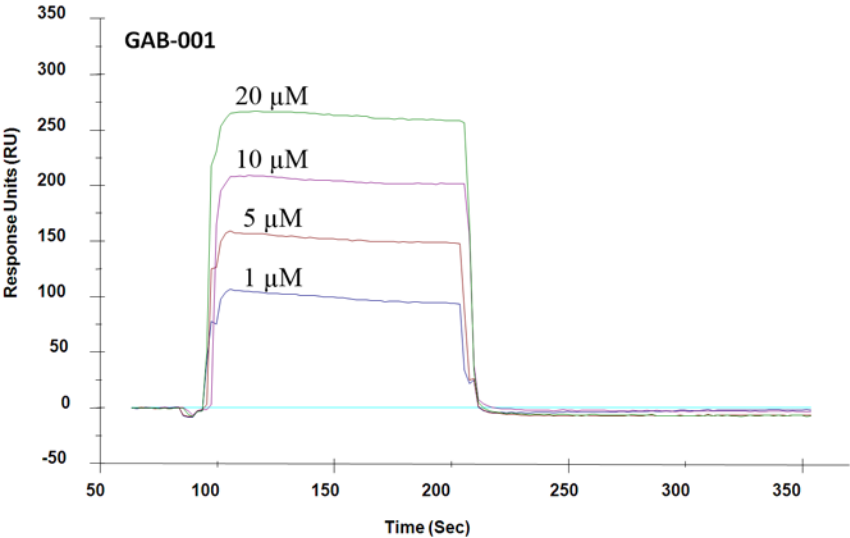
Figure S6. SPR of GAB-001, GAB-016 binding to GAB1 PH domain.
