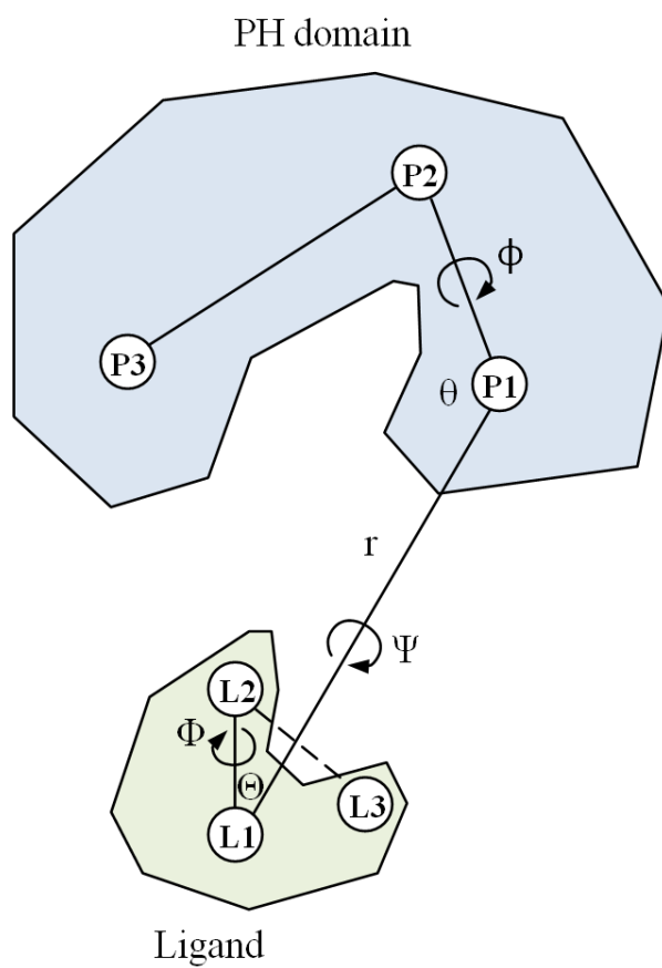
Figure S9. Schematic representation of frame of reference used to define the position and orientation restraints. To reduce the degrees of freedom, P1, P2, P3 and L1, L2, L3 were employed to represent the coordinates of the protein and the ligand, respectively, as described in Method S1 .
