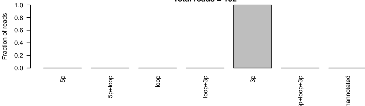
D) PPB Case 14 cell line miRNA sequencing ID=MI0000290_1;accession_number=MI0000290;Name=hsa-mir-214 Total reads = 102
