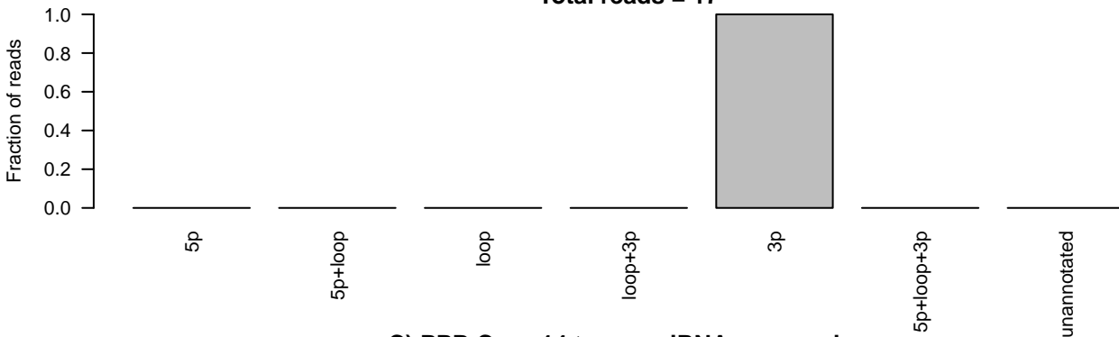
C) PPB Case 14 tumor miRNA sequencing ID=MI0000103_1;accession_number=MI0000103;Name=hsa-mir-101-1 Total reads = 48
