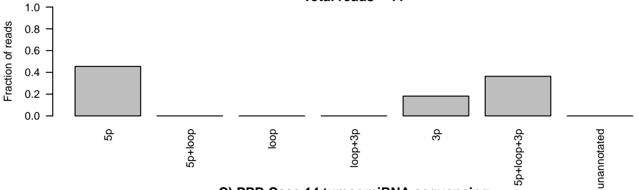
C) PPB Case 14 tumor miRNA sequencing ID=MI0000813_1;accession_number=MI0000813;Name=hsa-mir-324 Total reads = 3
