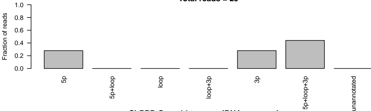
C) PPB Case 14 tumor miRNA sequencing ID=MI0000815_1;accession_number=MI0000815;Name=hsa-mir-339 Total reads = 31
