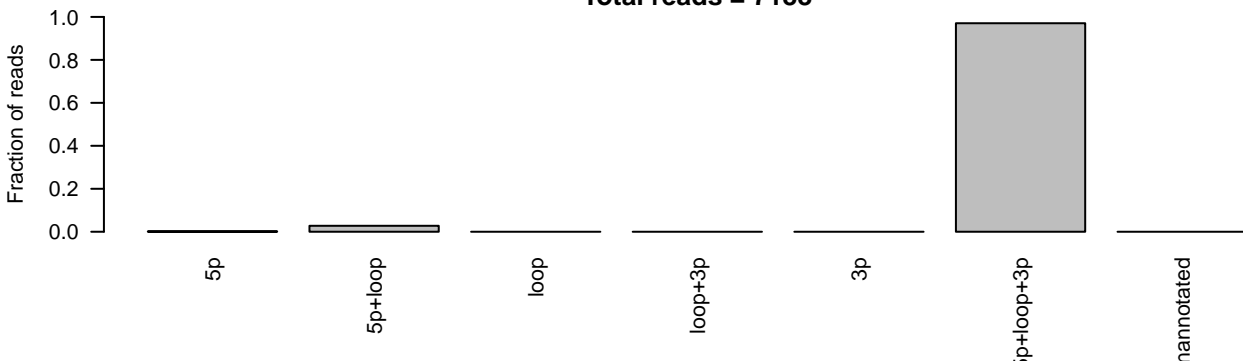
D) PPB Case 14 cell line miRNA sequencing ID=MI0015997_1;accession_number=MI0015997;Name=hsa-mir-3607 Total reads = 7188
