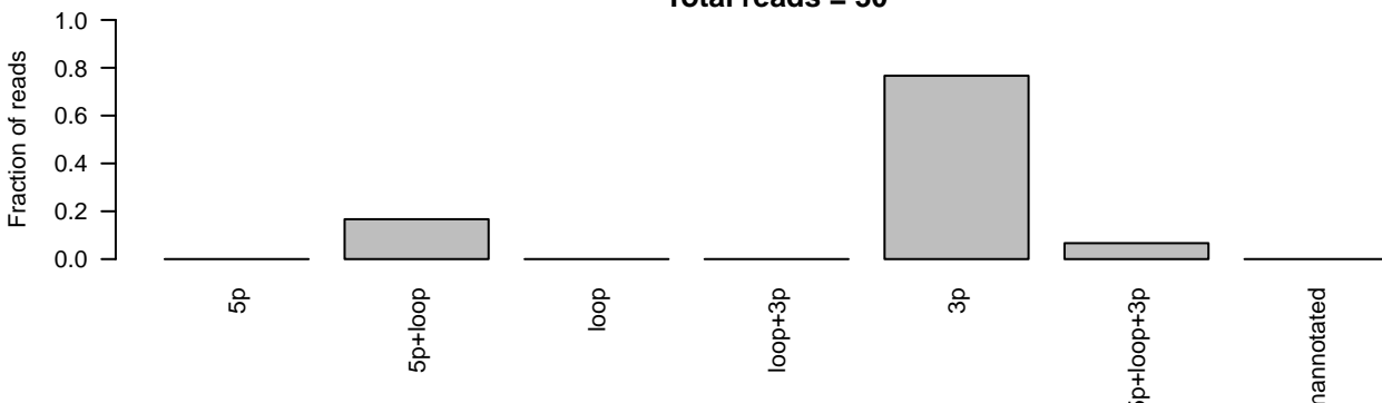
D) PPB Case 14 cell line miRNA sequencing ID=MI0001445_1;accession_number=MI0001445;Name=hsa-mir-423 Total reads = 30
