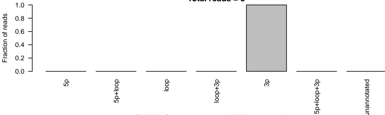
C) PPB Case 14 tumor miRNA sequencing ID=MI0000812_1;accession_number=MI0000812;Name=hsa-mir-331 Total reads = 7
