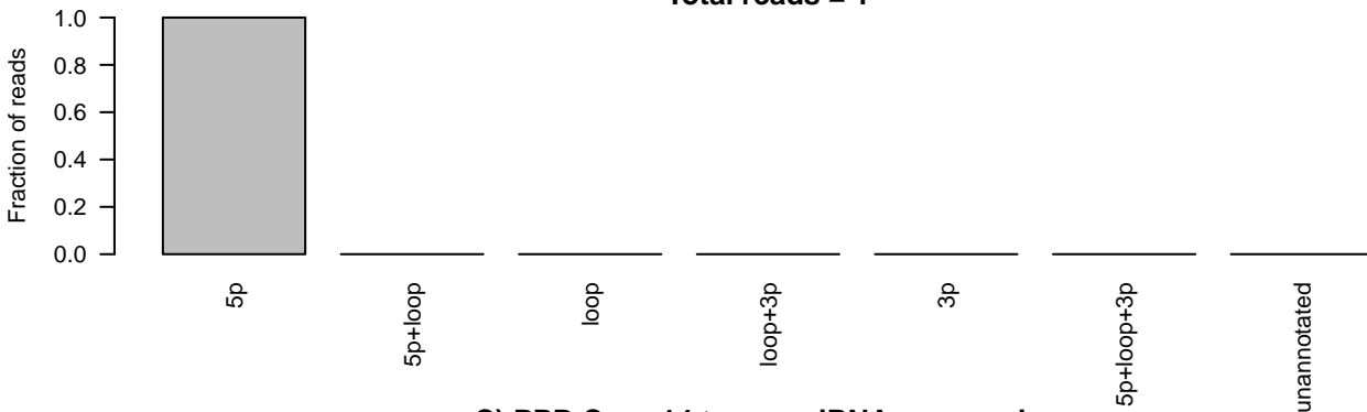
C) PPB Case 14 tumor miRNA sequencing ID=MI0003591_1;accession_number=MI0003591;Name=hsa-mir-584 Total reads = 0
