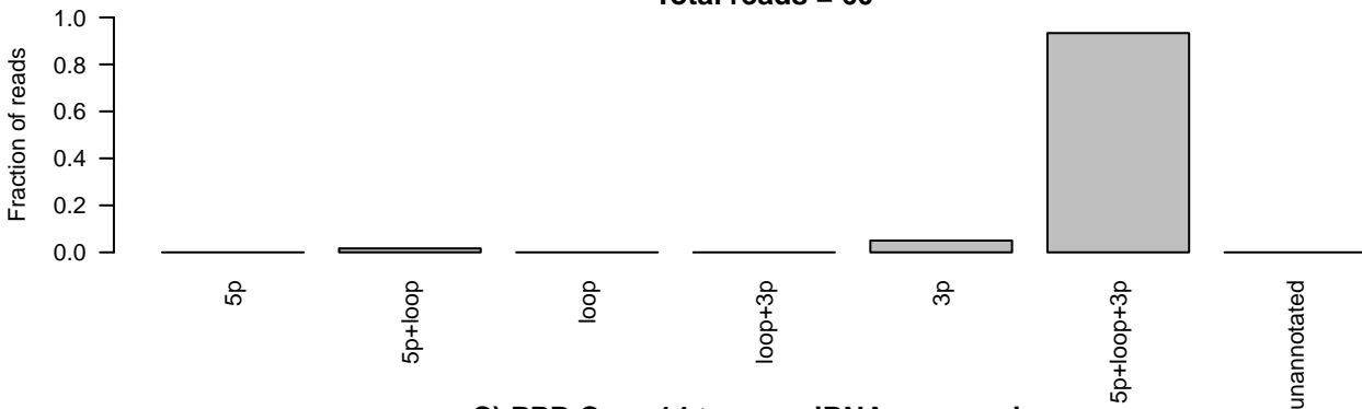
C) PPB Case 14 tumor miRNA sequencing ID=MI0000439_1;accession_number=MI0000439;Name=hsa-mir-23b Total reads = 65
