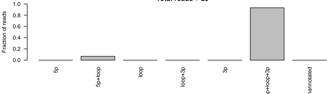
D) PPB Case 14 cell line miRNA sequencing ID=MI0003529_1;accession_number=MI0003529;Name=hsa-mir-376a-2 Total reads = 29
