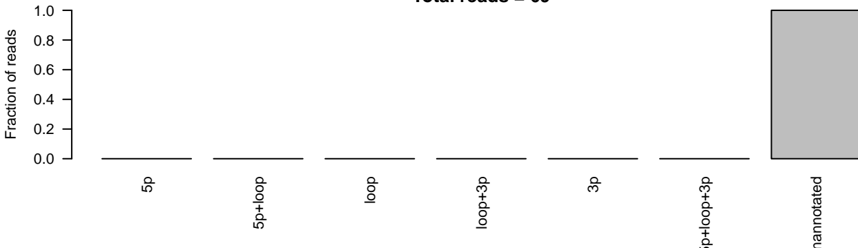
D) PPB Case 14 cell line miRNA sequencing ID=MI0005565_1;accession_number=MI0005565;Name=hsa-mir-543 Total reads = 69
