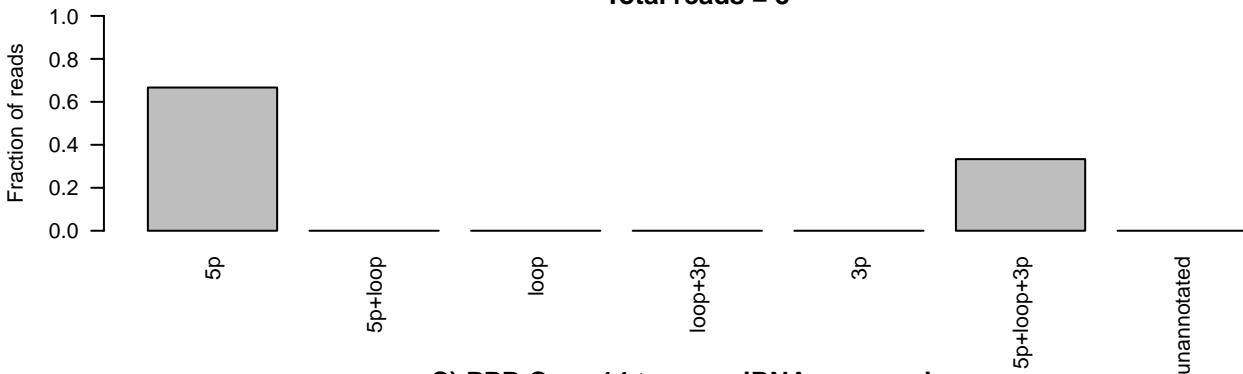
C) PPB Case 14 tumor miRNA sequencing ID=MI0000825_1;accession_number=MI0000825;Name=hsa-mir-345 Total reads = 5
