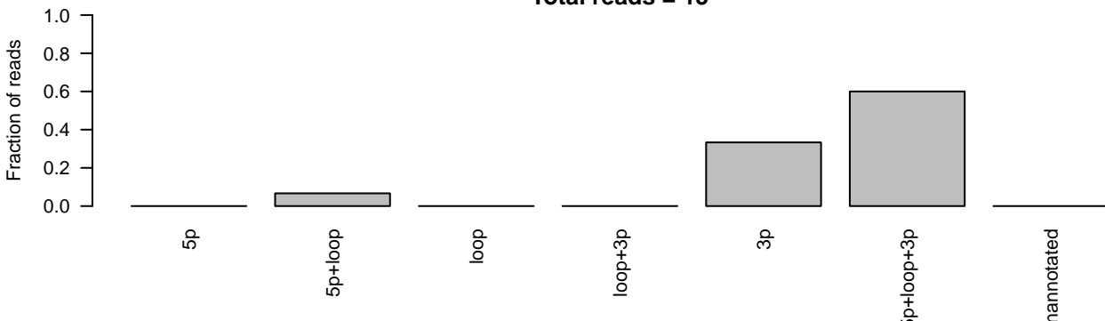
D) PPB Case 14 cell line miRNA sequencing ID=MI0000472_1;accession_number=MI0000472;Name=hsa-mir-127 Total reads = 15
