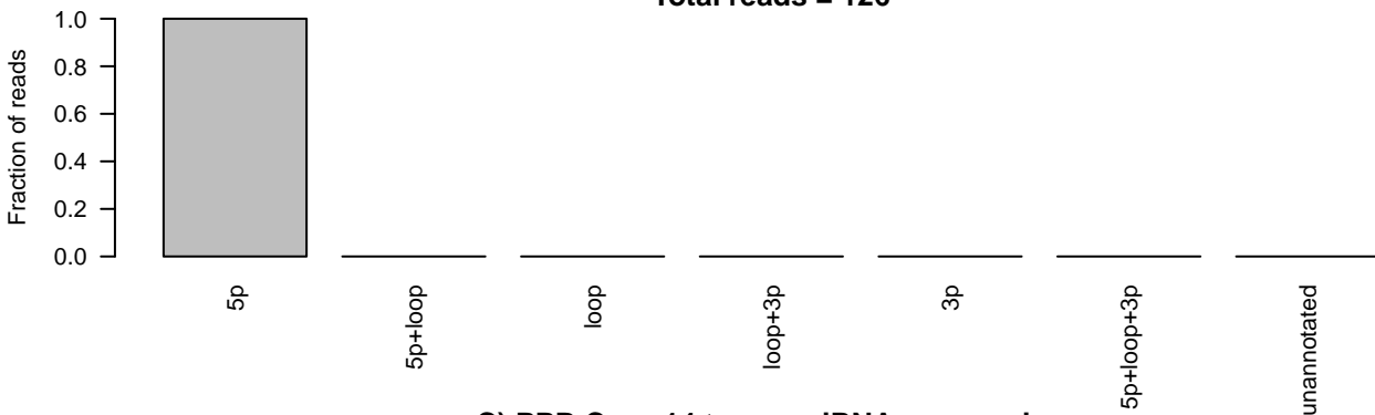
C) PPB Case 14 tumor miRNA sequencing ID=MI0000113_1;accession_number=MI0000113;Name=hsa-mir-106a Total reads = 2
