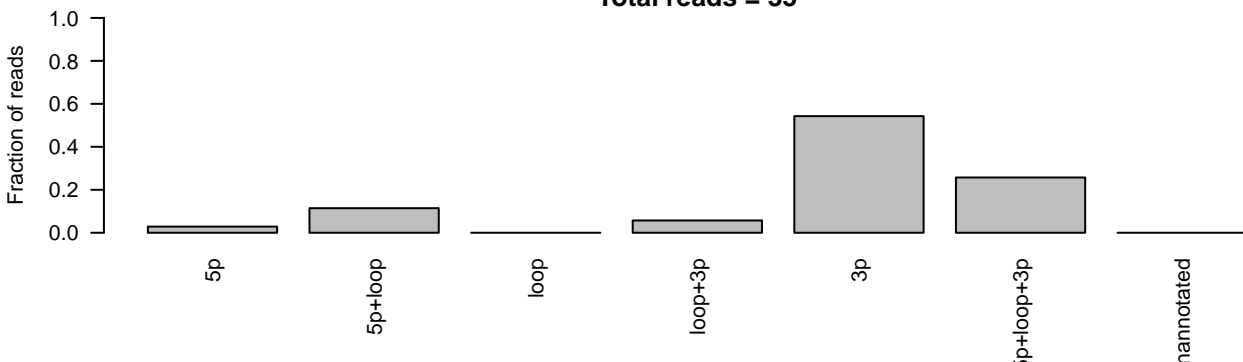
D) PPB Case 14 cell line miRNA sequencing ID=MI0003132_1;accession_number=MI0003132;Name=hsa-mir-493 Total reads = 35
