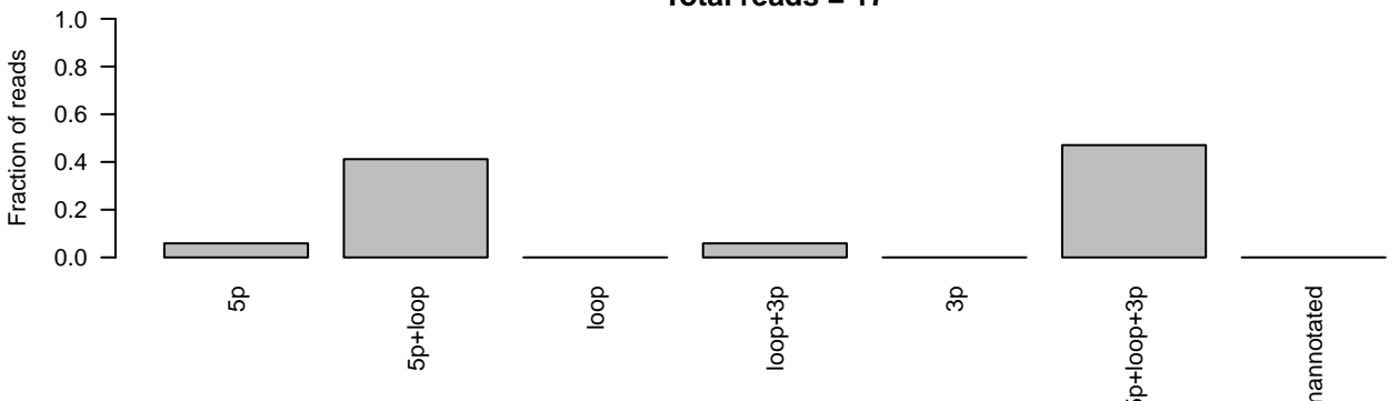
D) PPB Case 14 cell line miRNA sequencing ID=MI0000270_1;accession_number=MI0000270;Name=hsa-mir-181b-1 Total reads = 17
