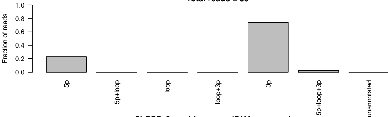
C) PPB Case 14 tumor miRNA sequencing ID=MI0000078_1;accession_number=MI0000078;Name=hsa-mir-22 Total reads = 10
