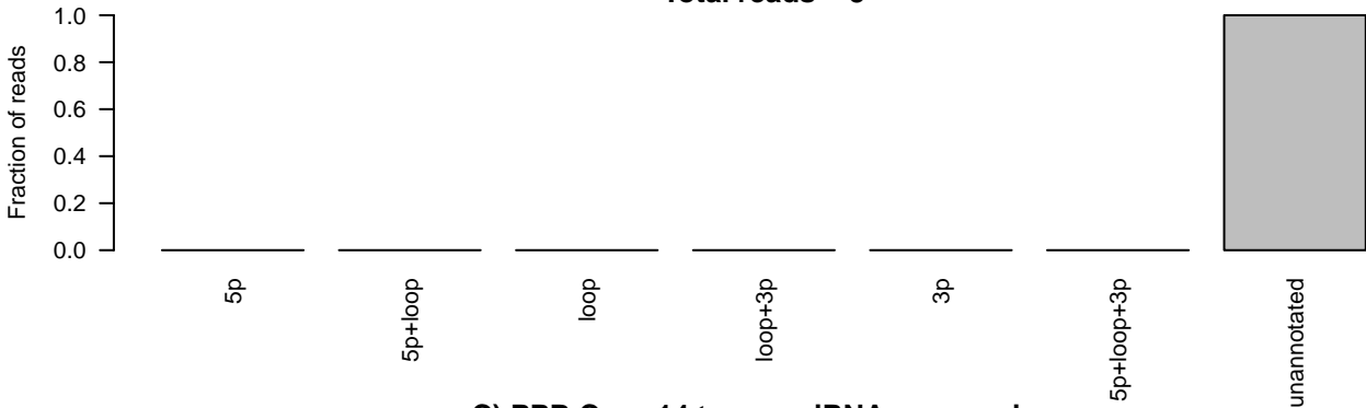
C) PPB Case 14 tumor miRNA sequencing ID=MI0000464_1;accession_number=MI0000464;Name=hsa-mir-153-2 Total reads = 1
