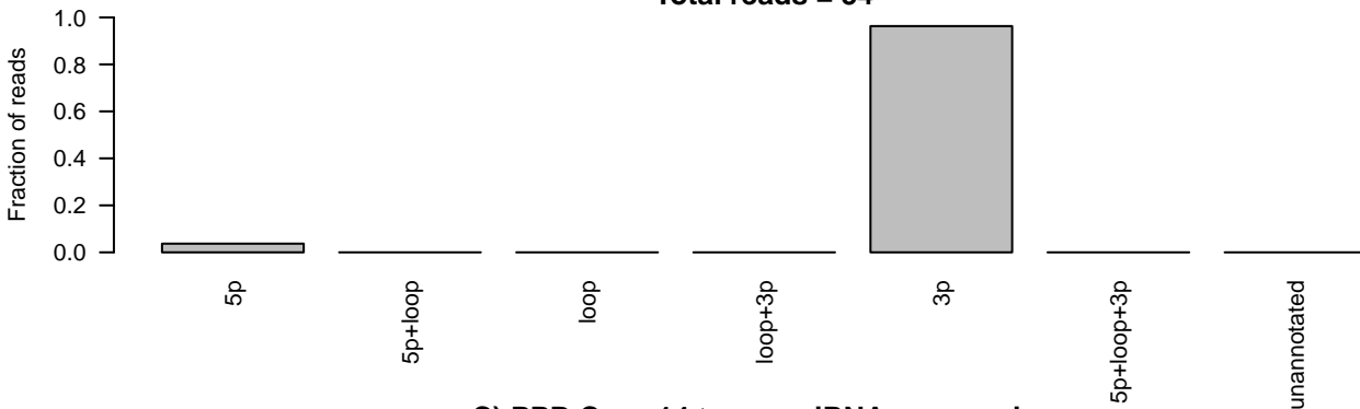
C) PPB Case 14 tumor miRNA sequencing ID=MI0000290_1;accession_number=MI0000290;Name=hsa-mir-214 Total reads = 133
