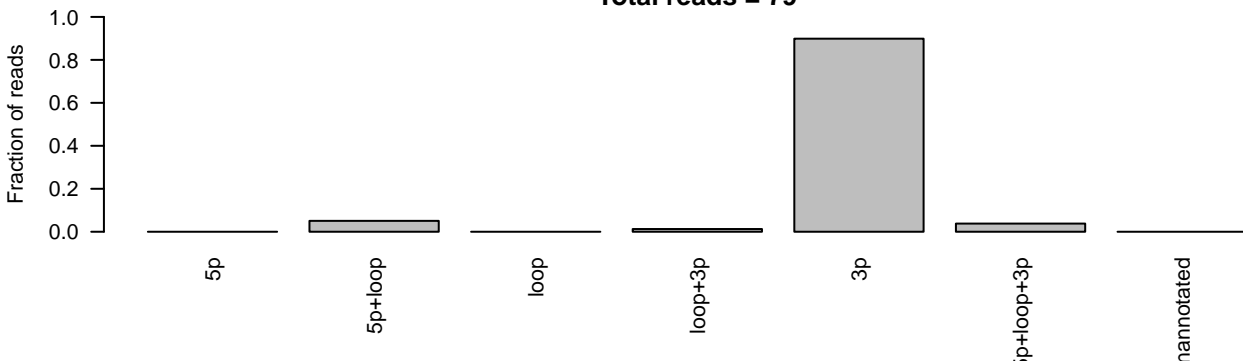
D) PPB Case 14 cell line miRNA sequencing ID=MI0000085_1;accession_number=MI0000085;Name=hsa-mir-27a Total reads = 79
