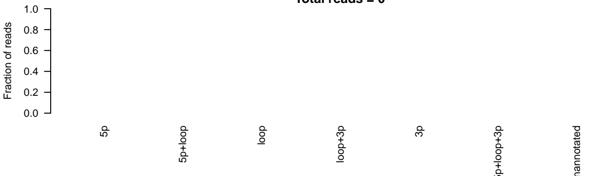
D) PPB Case 14 cell line miRNA sequencing ID=MI0000265_1;accession_number=MI0000265;Name=hsa-mir-7-3 Total reads = 0
