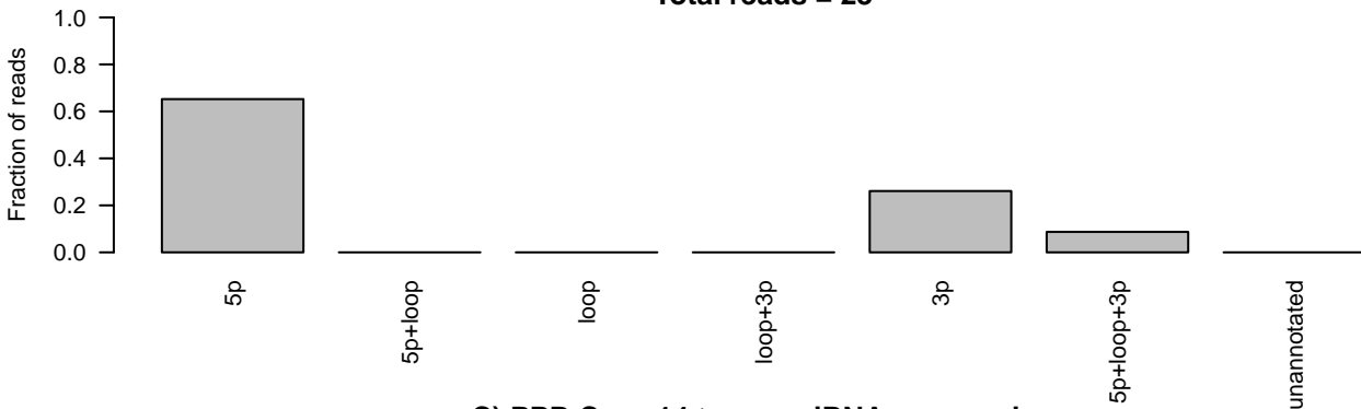
C) PPB Case 14 tumor miRNA sequencing ID=MI0003132_1;accession_number=MI0003132;Name=hsa-mir-493 Total reads = 150
