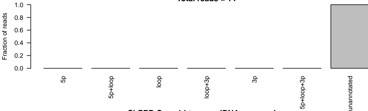
C) PPB Case 14 tumor miRNA sequencing ID=MI0005568_1;accession_number=MI0005568;Name=hsa-mir-301b Total reads = 38
