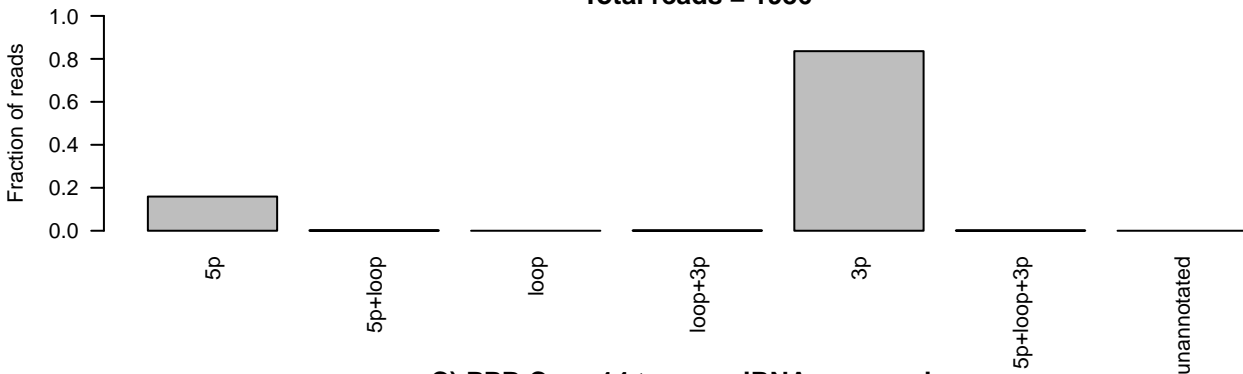
C) PPB Case 14 tumor miRNA sequencing ID=MI0000298_1;accession_number=MI0000298;Name=hsa-mir-221 Total reads = 6
