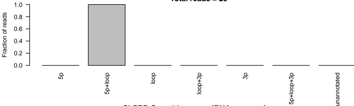
C) PPB Case 14 tumor miRNA sequencing ID=MI0016077_1;accession_number=MI0016077;Name=hsa-mir-3676 Total reads = 44
