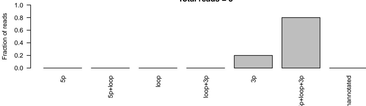
D) PPB Case 14 cell line miRNA sequencing ID=MI0000815_1;accession_number=MI0000815;Name=hsa-mir-339 Total reads = 5
