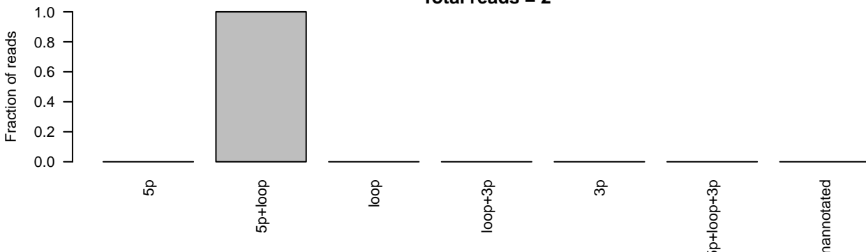
D) PPB Case 14 cell line miRNA sequencing ID=MI0000441_1;accession_number=MI0000441;Name=hsa-mir-30b Total reads = 2
