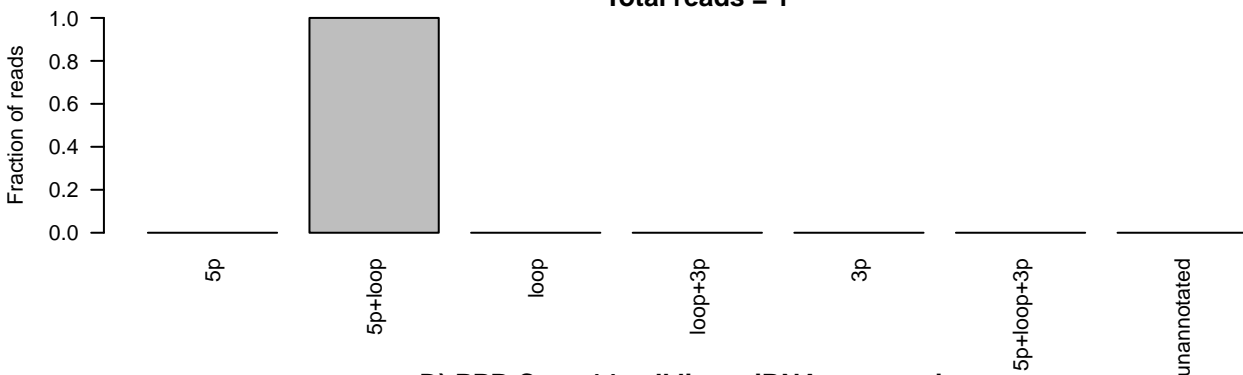
D) PPB Case 14 cell line miRNA sequencing ID=MI0003560_1;accession_number=MI0003560;Name=hsa-mir-92b Total reads = 1
