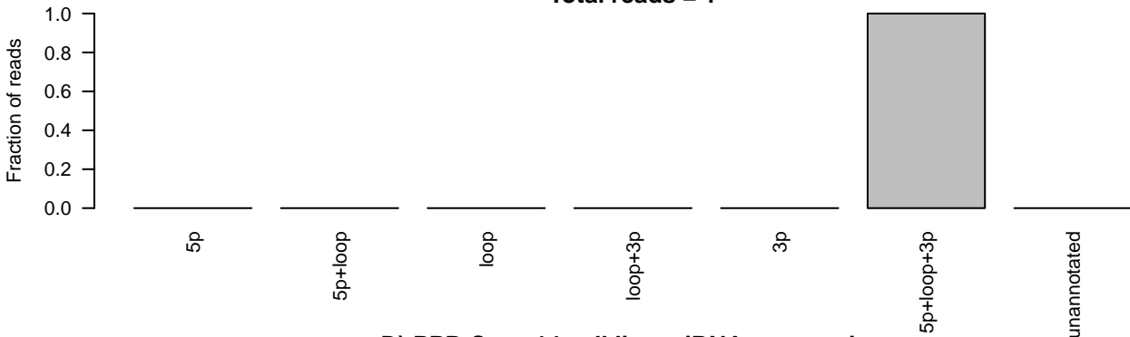
D) PPB Case 14 cell line miRNA sequencing ID=MI0003516_1;accession_number=MI0003516;Name=hsa-mir-545 Total reads = 4
