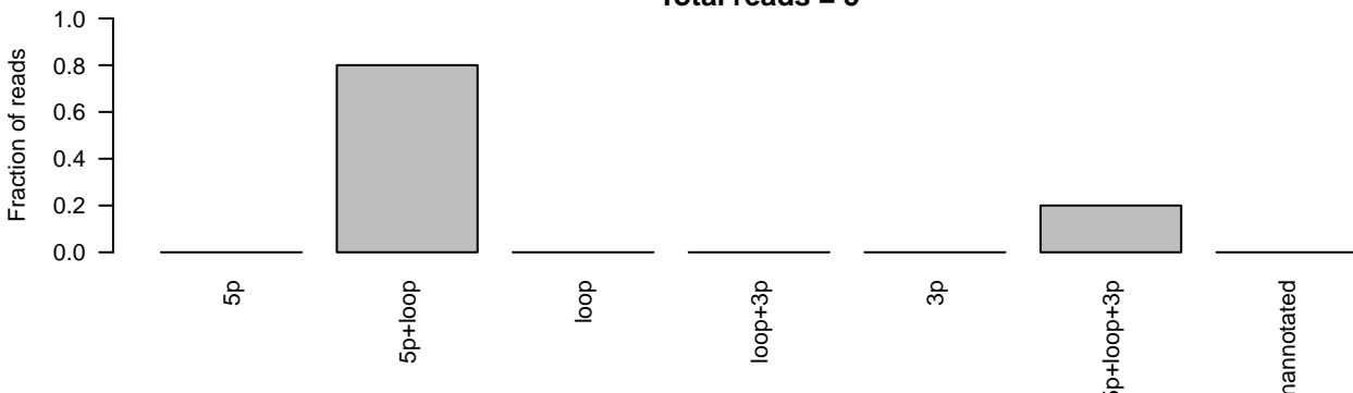
D) PPB Case 14 cell line miRNA sequencing ID=MI0000475_1;accession_number=MI0000475;Name=hsa-mir-136 Total reads = 5
