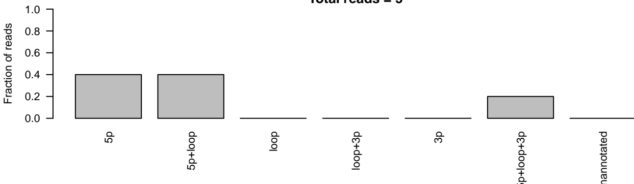
D) PPB Case 14 cell line miRNA sequencing ID=MI0000461_1;accession_number=MI0000461;Name=hsa-mir-145 Total reads = 5
