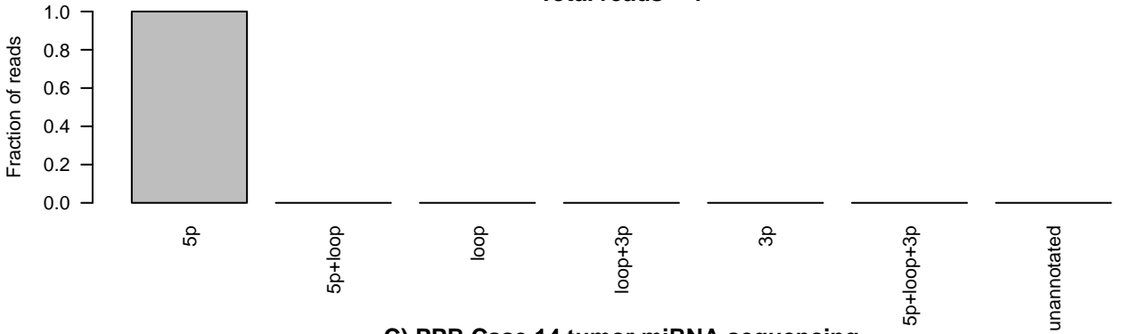
C) PPB Case 14 tumor miRNA sequencing ID=MI0003600_1;accession_number=MI0003600;Name=hsa-mir-550a-1 Total reads = 0
