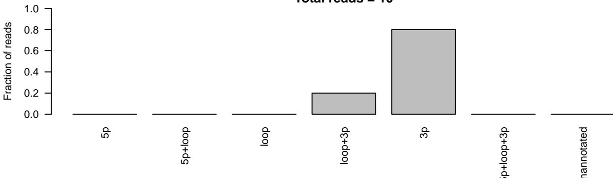
D) PPB Case 14 cell line miRNA sequencing ID=MI0016684_1;accession_number=MI0016684;Name=hsa-mir-374c Total reads = 10
