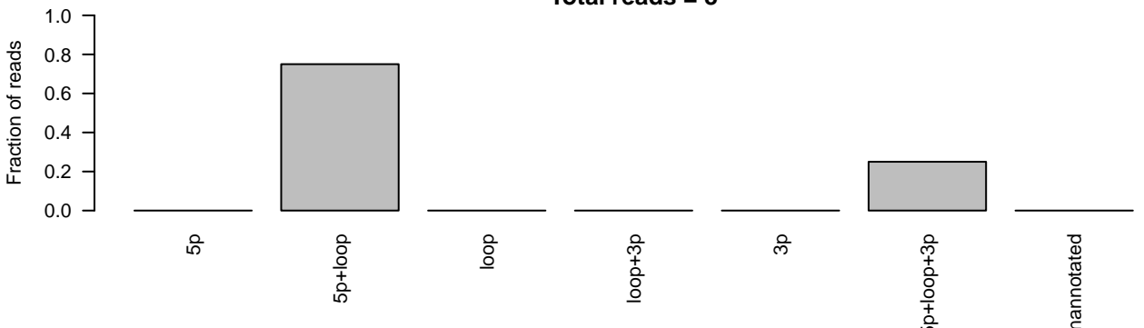
D) PPB Case 14 cell line miRNA sequencing ID=MI0001733_1;accession_number=MI0001733;Name=hsa-mir-452 Total reads = 8
