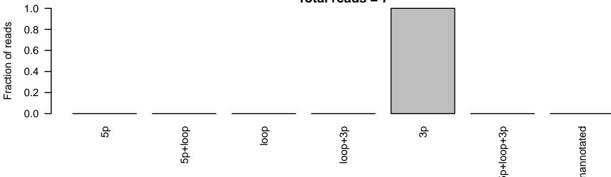
D) PPB Case 14 cell line miRNA sequencing ID=MI0000476_1;accession_number=MI0000476;Name=hsa-mir-138-1 Total reads = 7
