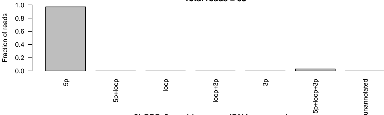
C) PPB Case 14 tumor miRNA sequencing ID=MI0000681_1;accession_number=MI0000681;Name=hsa-mir-155 Total reads = 0
