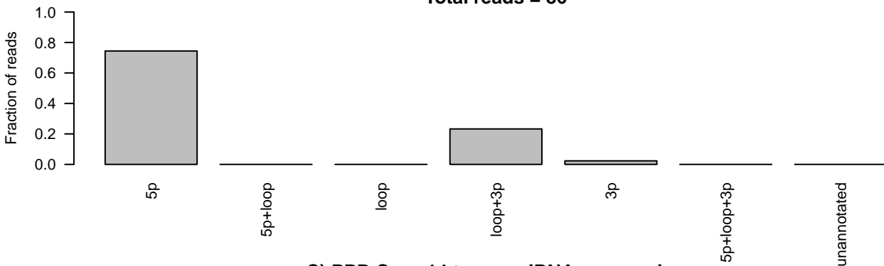
C) PPB Case 14 tumor miRNA sequencing ID=MI0014226_1;accession_number=MI0014226;Name=hsa-mir-3184 Total reads = 39
