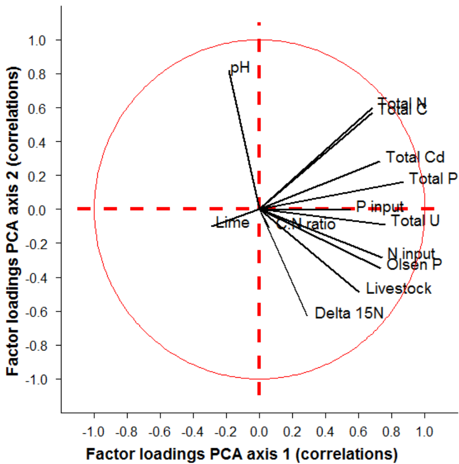
Figure S2. Factor loadings (correlations) on PCA axes 1 and 2 showing the dominant farmer input measures and soil biogeochemistry measures driving variation in land-use intensity across farms.
