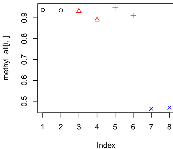
methyl NM_032040
