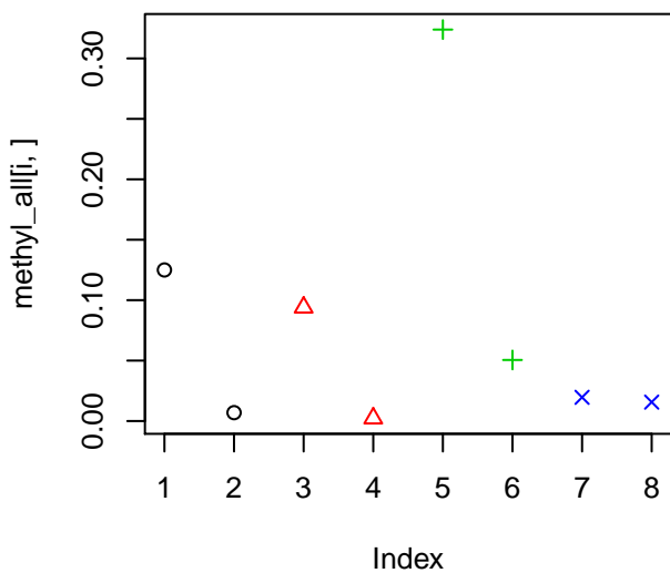
methyl NM_153608
