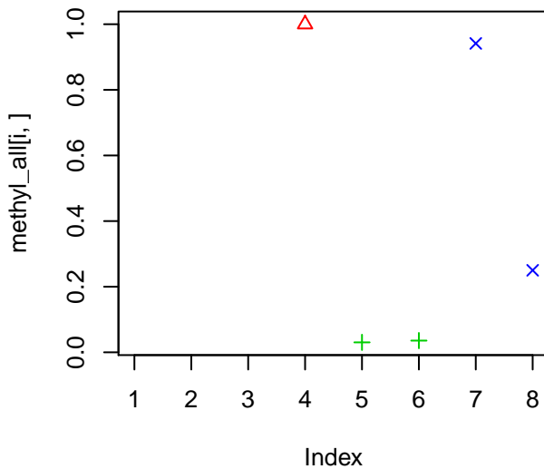
methyl NM_006762
