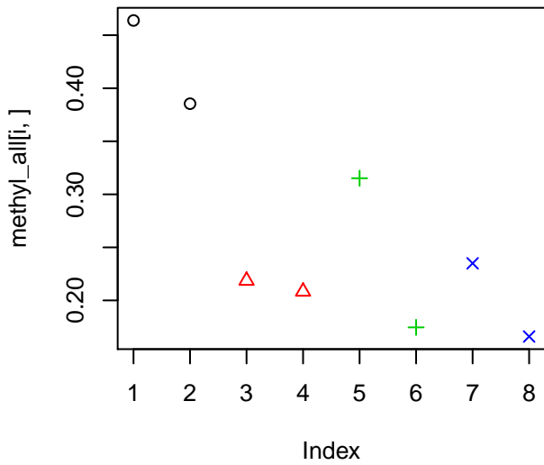
methyl NM_000201
