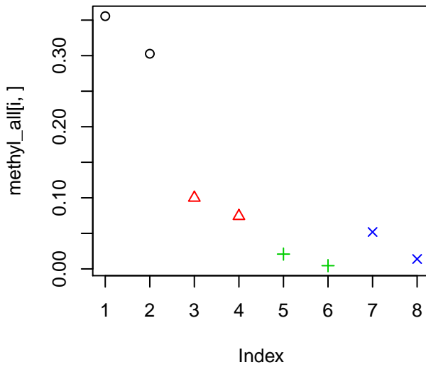
methyl NM_022164
