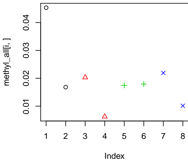
methyl NM_020182
