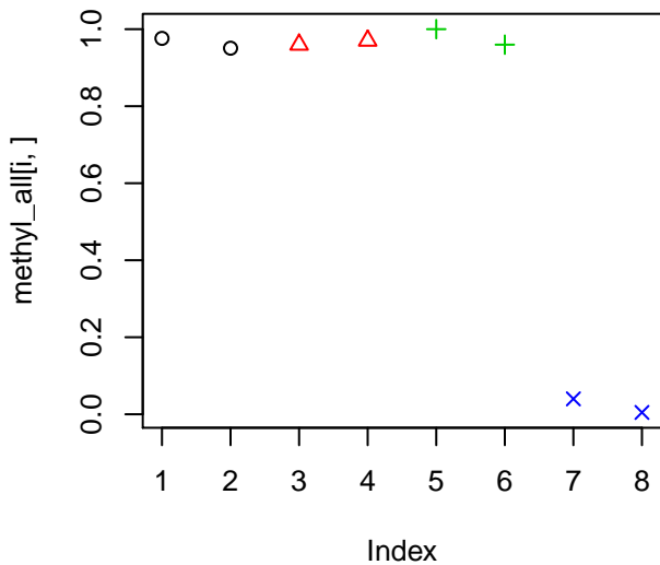
methyl NM_002145
