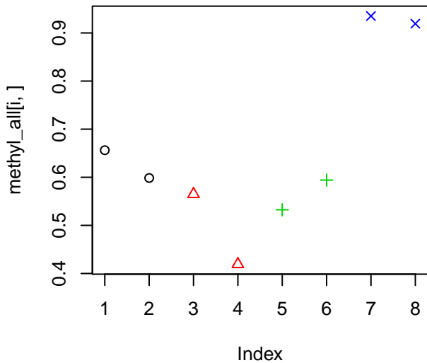
methyl NM_003781
