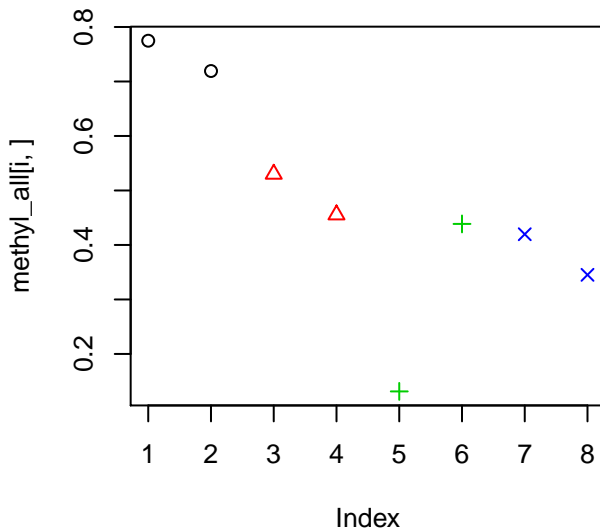
methyl NM_002996
