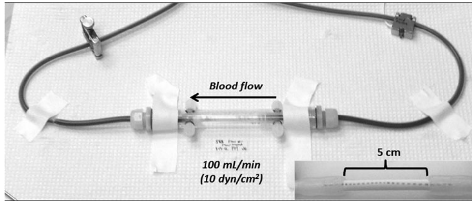
SUPPLEMENTARY FIG. S1. A cell-seeded ePTFE vascular graft connected to the baboon arteriovenous shunt loop. Vascular grafts 5 cm in length are connected to a silicone tubing (inset) for connection to the shunt loop. Blood flows from the femoral artery of the baboon, through the graft, and back into the femoral vein. The blood flow rate is monitored with a Transonic flow probe and held constant at 100 mL/min by a clamp downstream of the graft. ePTFE, expanded polytetrafluoroethylene.
