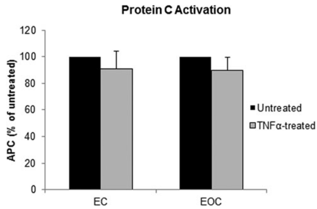
SUPPLEMENTARY FIG. S3. APC generation of TNF \alpha -treated ECs and EOCs normalized to untreated cells. Both ECs and EOCs consistently reduced protein C activation following TNF \alpha treatment, although the degree of TNF \alpha -induced reduction varied between donors. Decreases in protein C activation were not significant between untreated and treated (paired t -test, p=0.094 for ECs, p=0.10 for EOCs, n=8 , analysis performed before normalization). APC, activated protein C.
