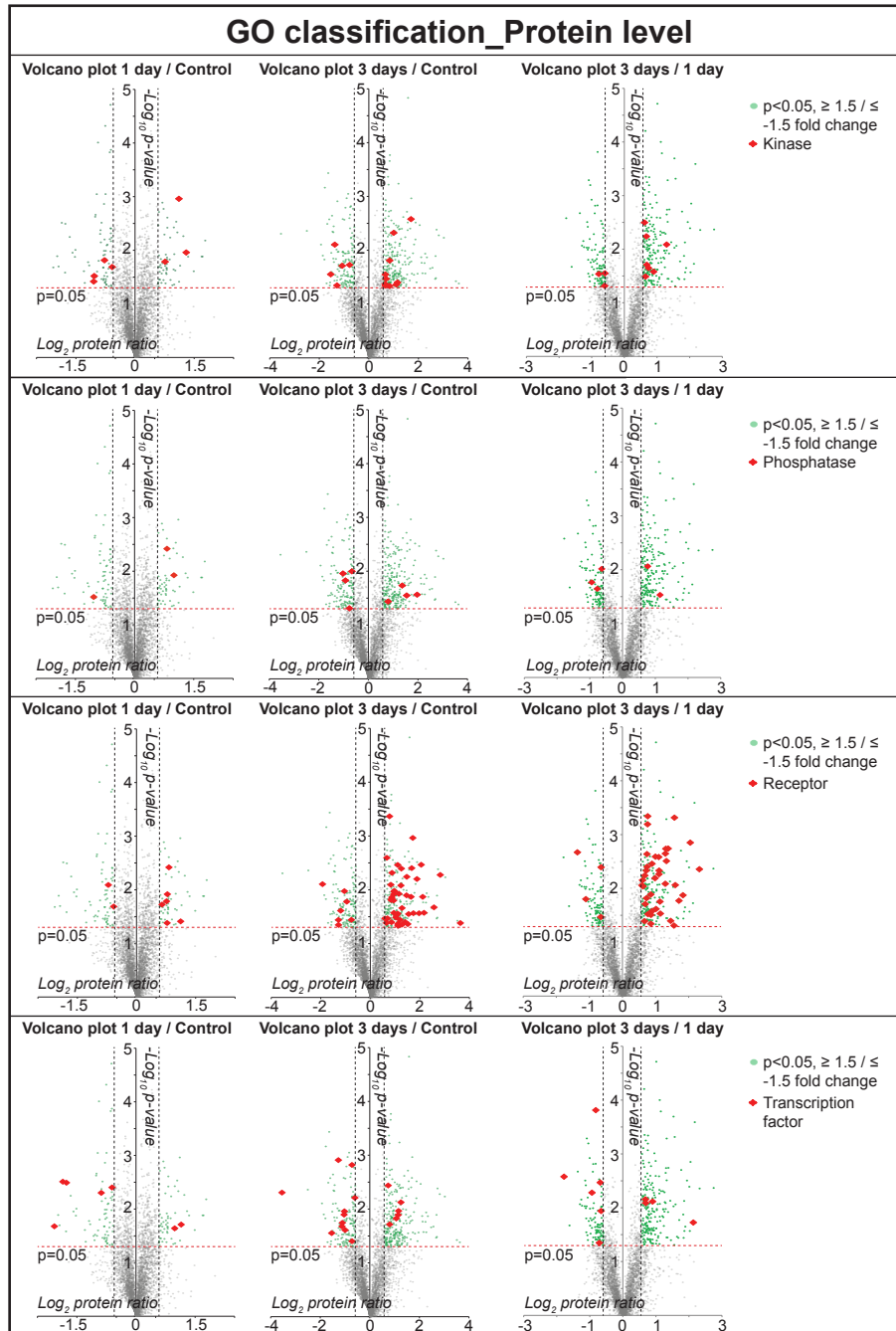
Figure S2. GO classification using Panther. Proteins belonging to the four categories (kinase; phosphatase; receptor; transcription factor) that are over-represented among the significant entries are labeled by a red diamond in each volcano plot at each time point.
