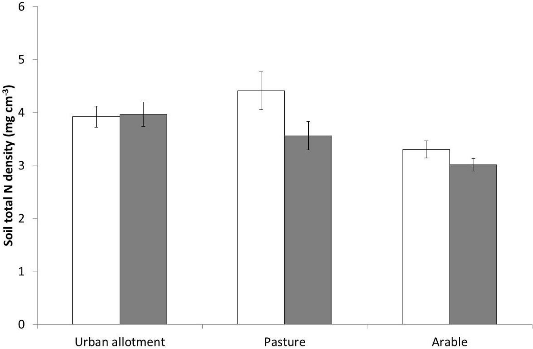
Fig. S1: Mean soil nitrogen density in urban allotment and agricultural soils: 0 – 7 cm depth represented by white bars; 7 – 14 cm indicated by grey bars. Error bars are \pm 1 standard error.
