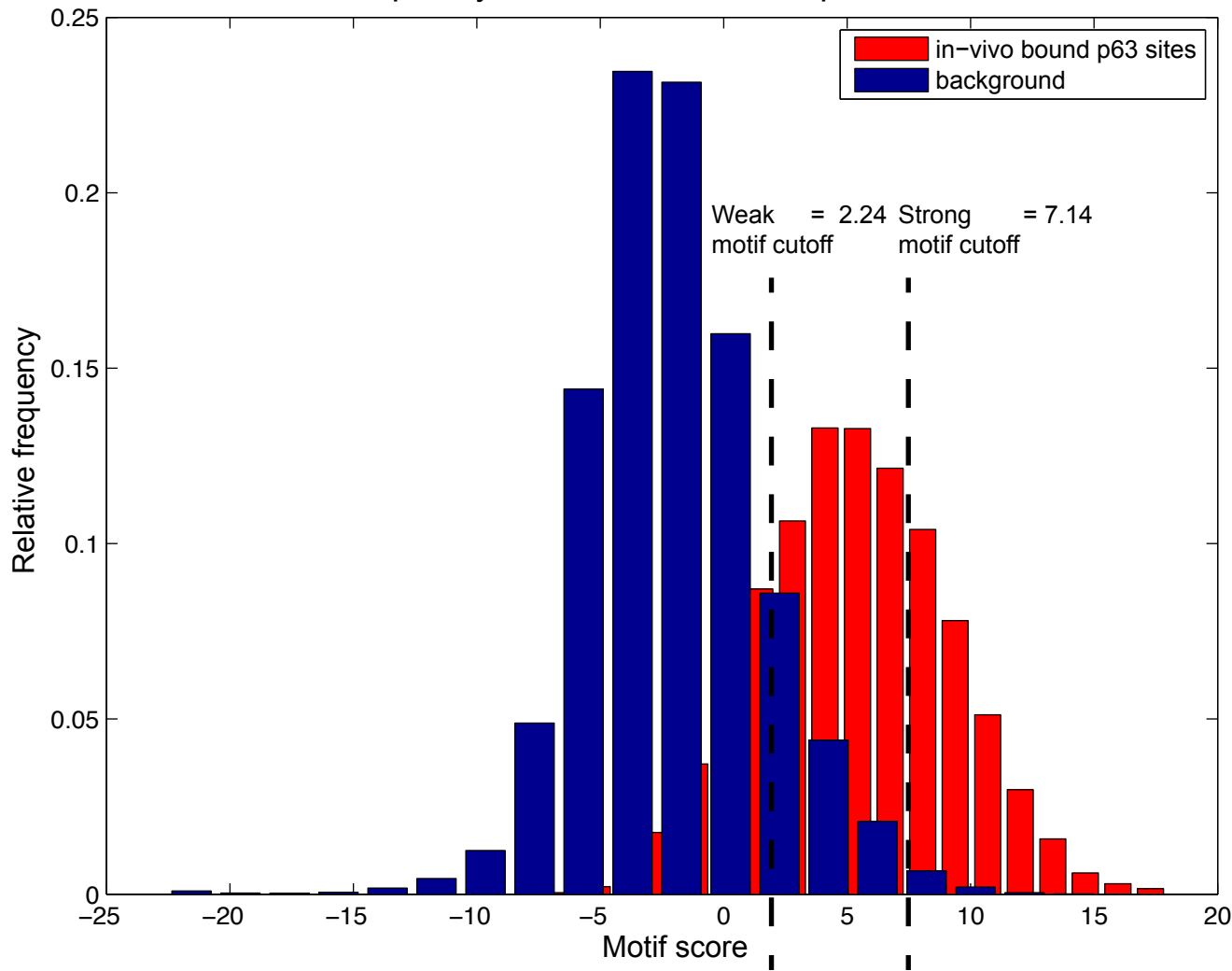
Frequency Distribution curve of p63 motif scores
