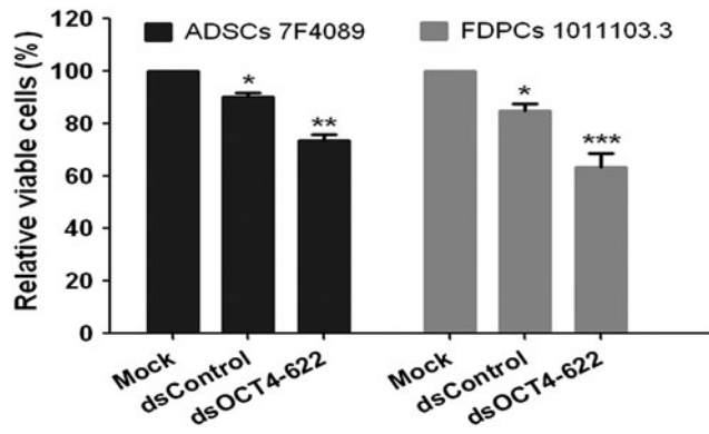
SUPPLEMENTARY FIG. S2. RNAa-mediated OCT4 activation inhibits cell viability of ADSCs and FDPCs. ADSCs 7F4089 and FDPCs 1011103.3 were transfected with the indicated dsRNAs at 50 nM. MTT assay was conducted 96 h following transfection. Results are plotted as the percentage of viable cells relative to mock transfections. n=3 . * P<0.05 ; ** P<0.01 ; *** P<0.001 .
