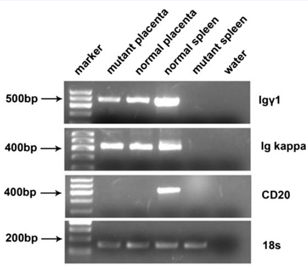
Supplementary Figure S6 RT-PCR showing the expression of IgG in mouse placentas. Igγ1 and Igκ were detected in placentas of mutant mouse, placentas of normal ICR mouse and spleen of normal ICR mouse. The spleen of mutant mouse served as negative control. 18s served as internal control. CD20 was detected to exclude the contamination of B lymphocytes.
