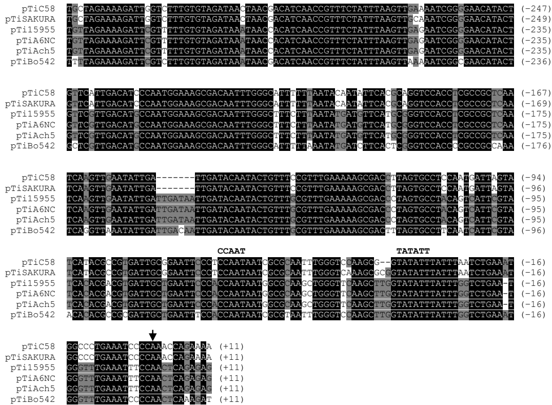
Figure S1 Alignment of IaaH promoters including the 5' untranslated regions from different A. tumefaciens strains.
