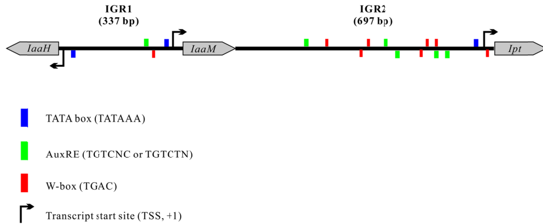
Figure S5 Cis -regulatory elements within IGR1 and IGR2.
