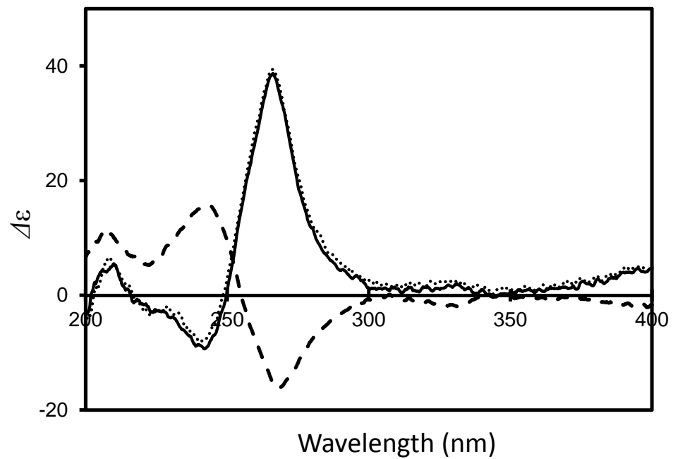
Supplemental Figure 1. CD spectra of 3'-hydroxyl-ε,ε-carotene-3-one isomers in ethanol. Peak A1, dashed line; Peak A2, solid line; (6'R,3R,6R)-3'-hydroxyl-ε,ε-carotene-3-one prepared from lactucaxanthin, dotted line.
