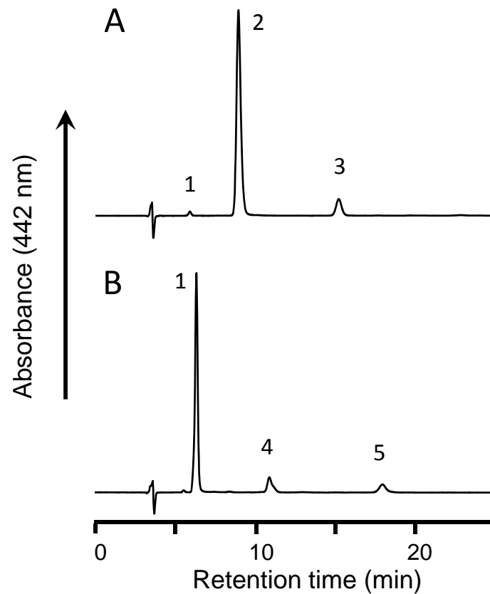
Supplemental Figure 3. Normal-phase HPLC profiles of extracts from incubation mixtures of lutein (A) and zeaxanthin (B) with liver postmitochondrial fraction after a prolonged incubation. 1, \epsilon,\epsilon -carotene-3,3'-dione; 2, 3'-hydroxyl- \epsilon,\epsilon -carotene-3-one; 3, lutein; 4, 3-hydroxyl- \beta,\epsilon -carotene-3'-one; 5, zeaxanthin.
