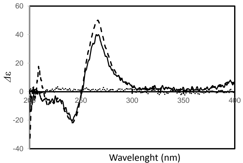
Supplemental Figure 4. CD spectra of \epsilon,\epsilon -carotene-3,3'-dione isomers in ethanol. Peak E1, dotted line; Peak E2, solid; (6R,6'R) - \epsilon,\epsilon -carotene-3,3'-dione prepared from lactucaxanthin, dashed line.
