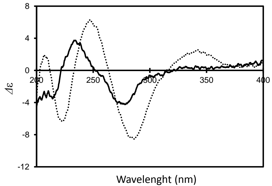
Supplemental Figure 5. CD spectra of \beta -cryptoxanthin (dotted line) and 3-hydroxyl- \beta,\epsilon -carotene-3'-one isolated from the reaction mixture of zeaxanthin with liver postmitochondrial fraction (solid line), in ethanol.
