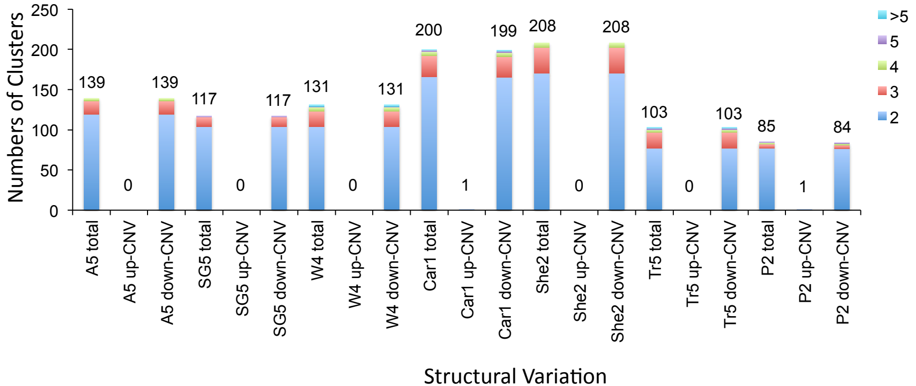
Figure S4. Clusters of copy number variants in switchgrass. The number of clusters of total, up-, and down-copy number variants (CNV) for seven switchgrass genotypes, including three lowland (A5, SG5-1 and W4) and four upland ecotypes (Car1, She2, Tr5 and P2). The total number of clusters for each genotype is listed at the top of the bar.
