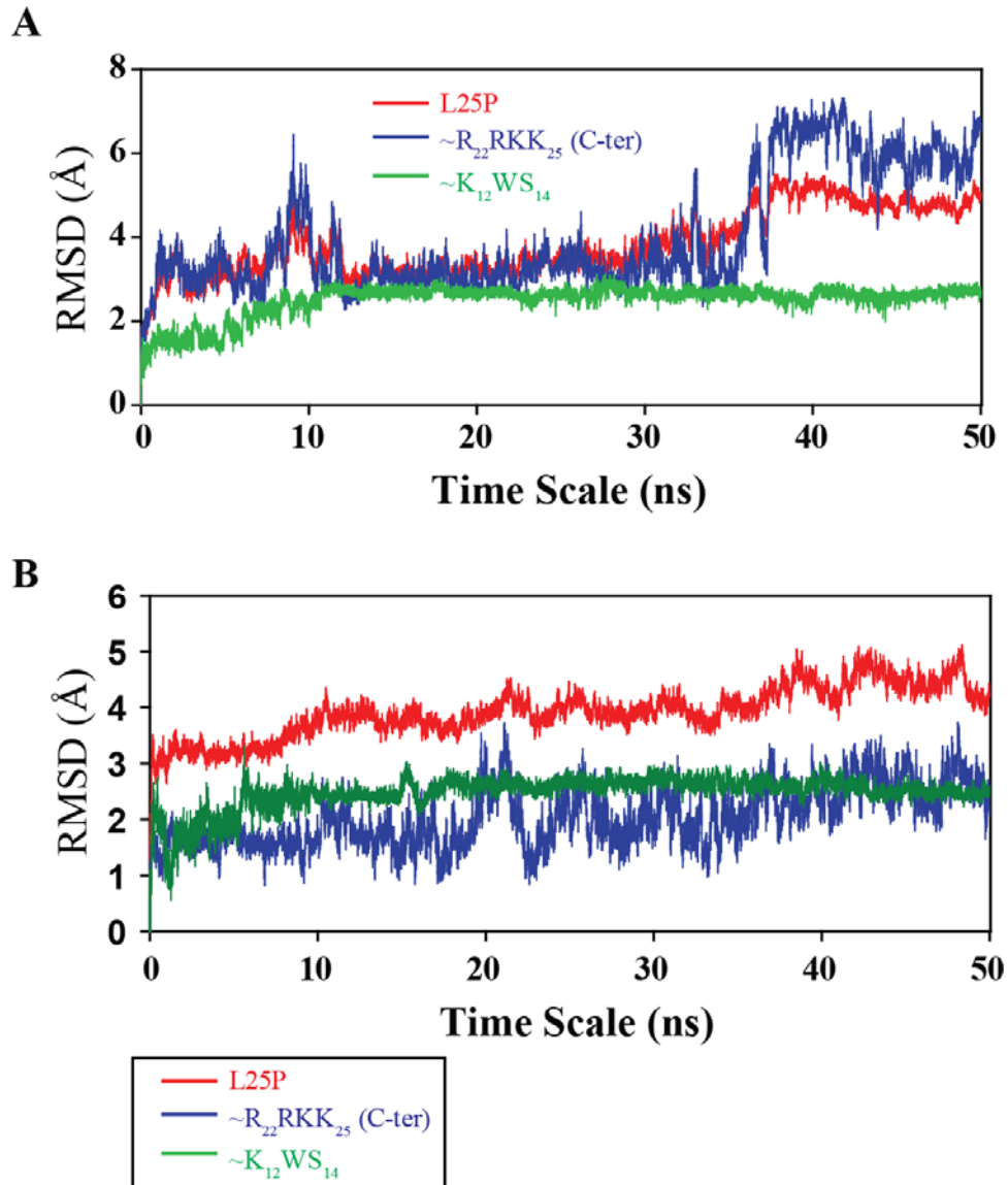
Figure S1. RMSD plot for a helical conformation of L25P (A) and a random-coil (B) in POPC bilayer.
