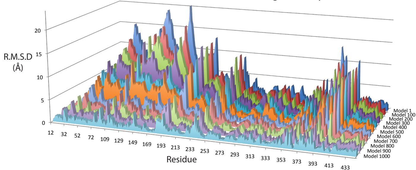
c) Per C \alpha R.M.S.D. of CDA-C1 MD simulation targeted to TycC conformation
