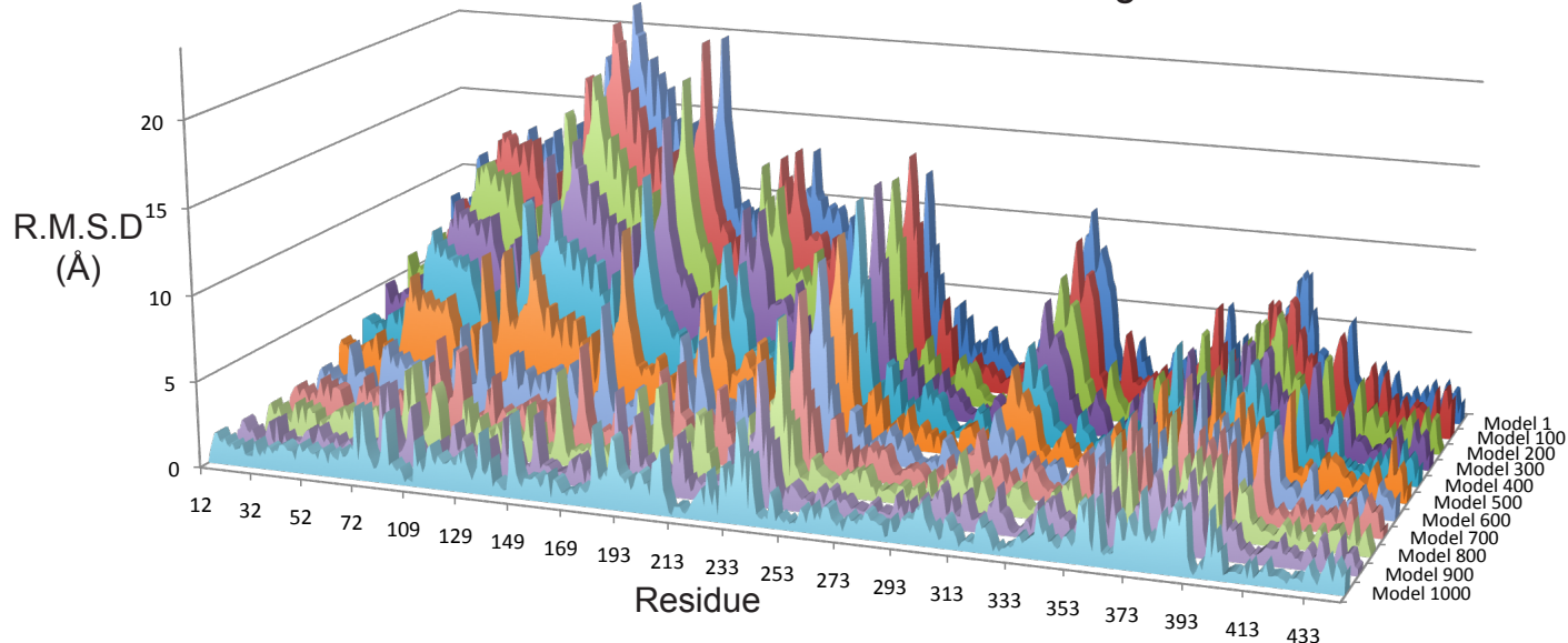
a) Per C \alpha R.M.S.D of CDA-C1 MD simulation targeted to SrfAC conformation
