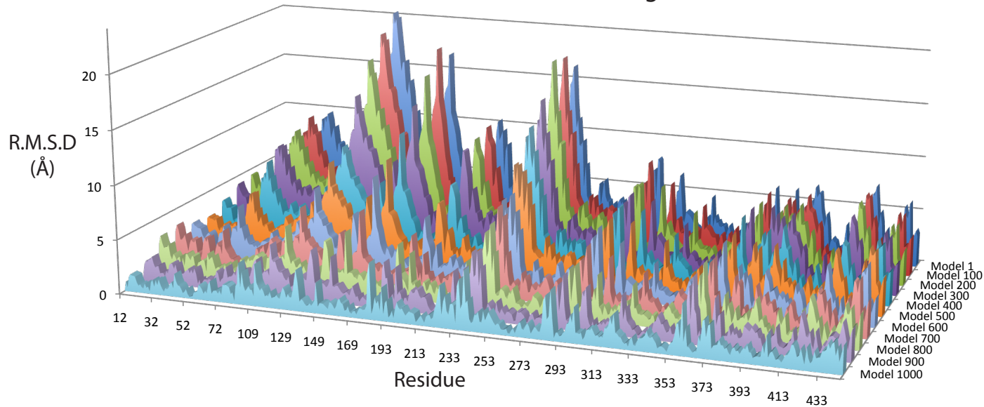
b) Per C \alpha R.M.S.D. of CDA-C1 MD simulation targeted to VibHh conformation
