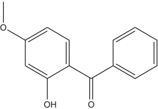
2-hydroxy-4-methoxybenzophenone
