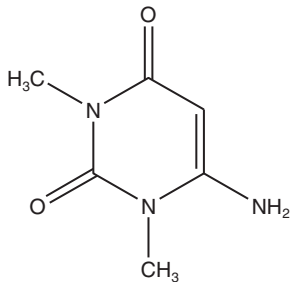
1,3-dimrthyluracil
