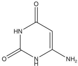
6 aminouracil
