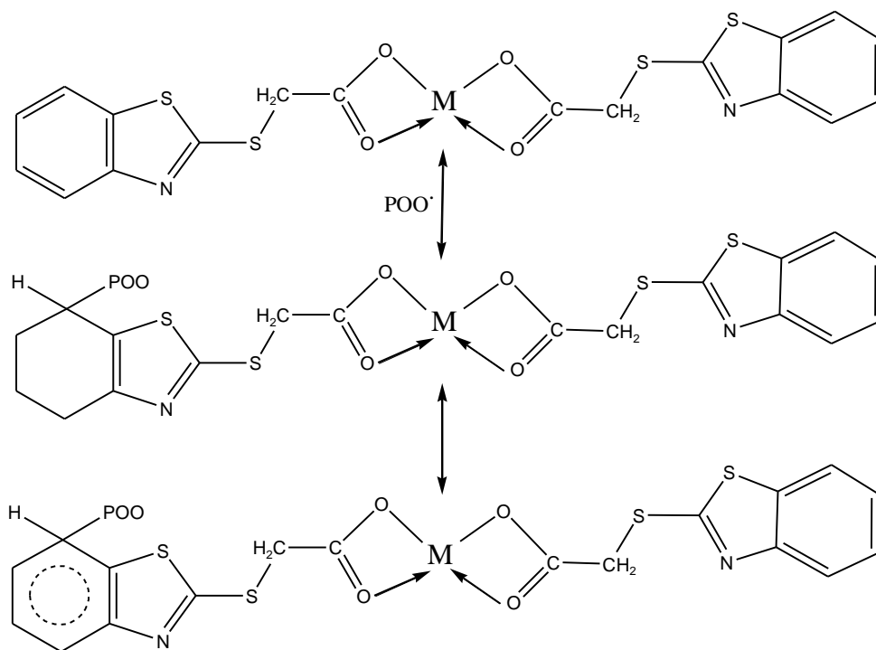
Scheme (7) Suggested mode of photostabilization by carboxylate complexes as radical scavengers.
