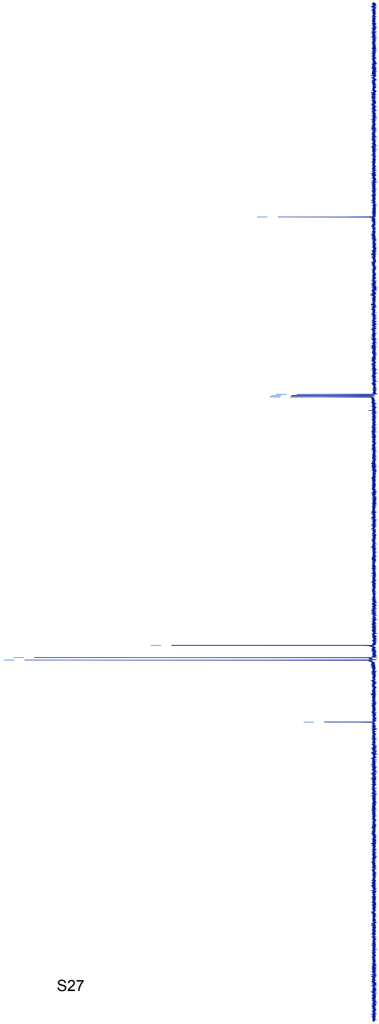
Scheme 2, 3a, X=Br
