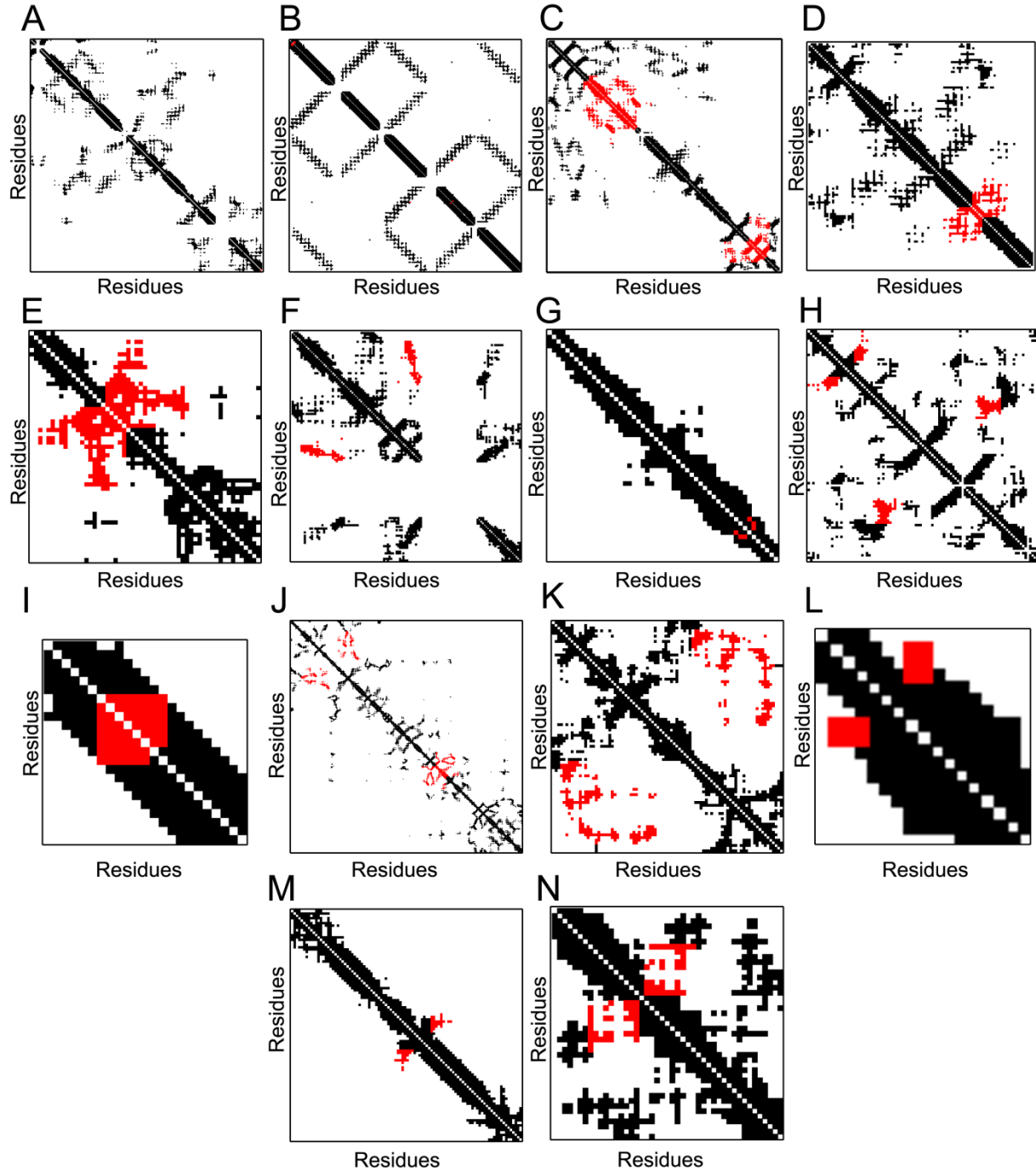
Supplement Figure S3. Contact map of HIV proteins during molecular dynamic simulations. Panel (A-N) represent CA, GP41, IN, MA, NC, NEF, P6, PR, REV, RT, TAT, VIF, VPR, and VPU respectively. The red regions are the protein sectors. For TAT and VPR, only the top ten coevolving residues were marked.
