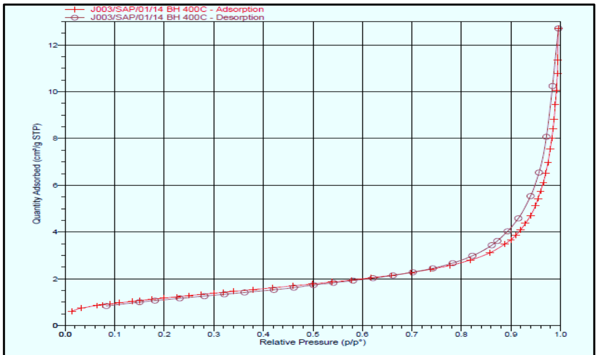
Fig. 2. N 2 adsorption-desorption isotherm of C. polygonides ash
