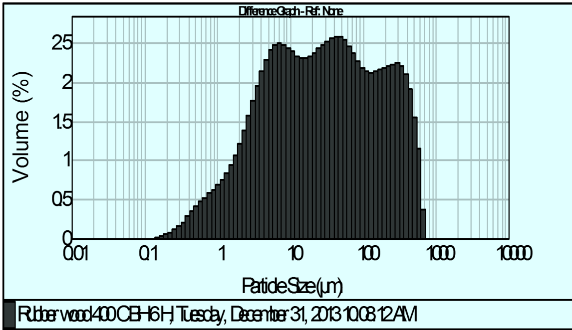
Fig. 1. Particle size of C. polygonides ash.
