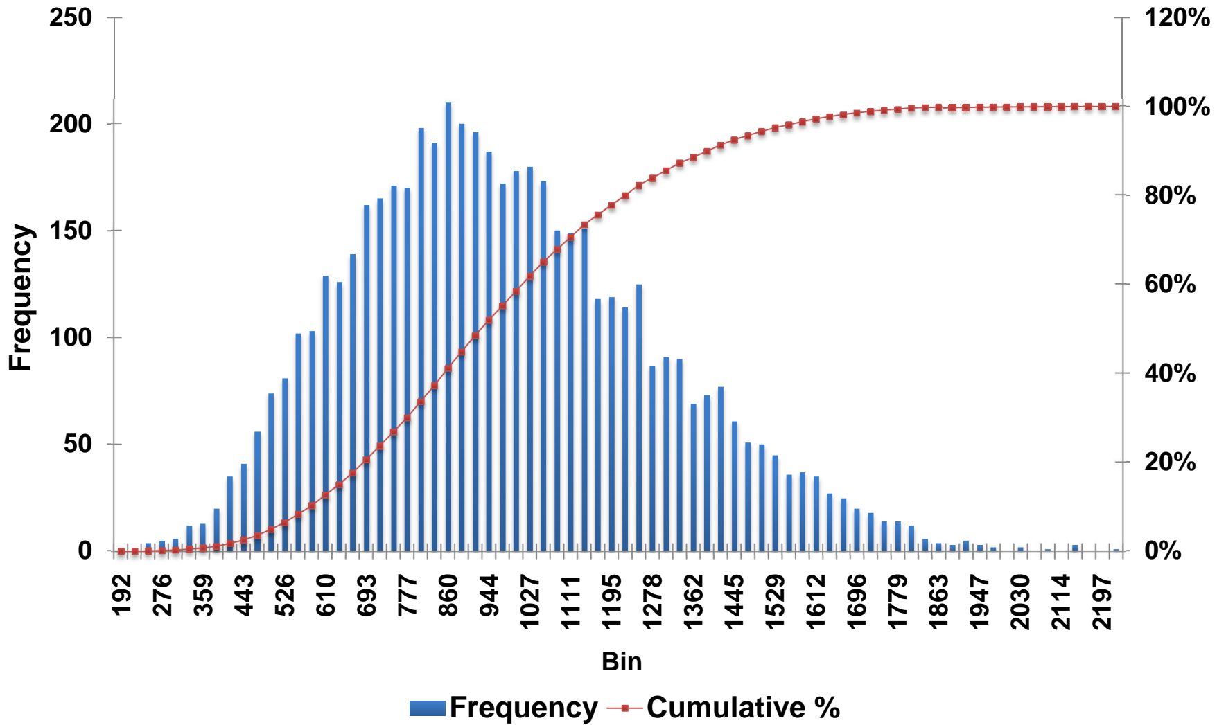
Histogram of CNV counts based on QuantiSNP (autosomes)
