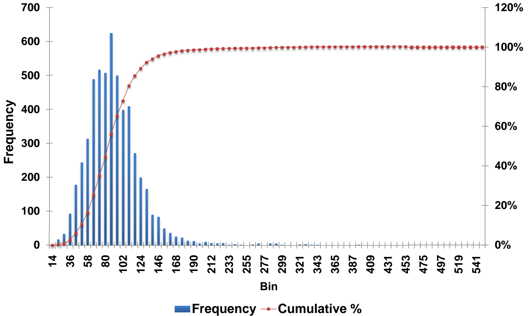
Histogram of CNV counts based on GNOSIS (autosomes)
