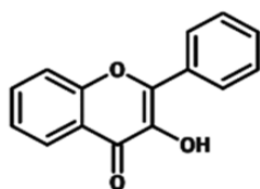
3-hydroxyflavone
