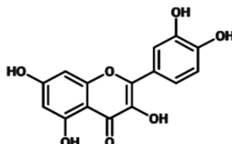
Quercetin
