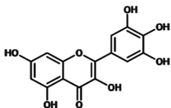
Myricetin
