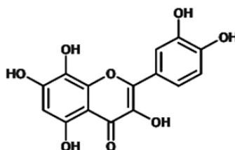
Gossypetin
