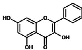
Galangin
