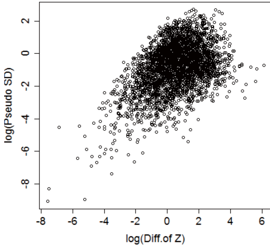
Figure S1. A scatter plot of the estimated pseudo variances and the difference of modified z-scores in the training experiments.
