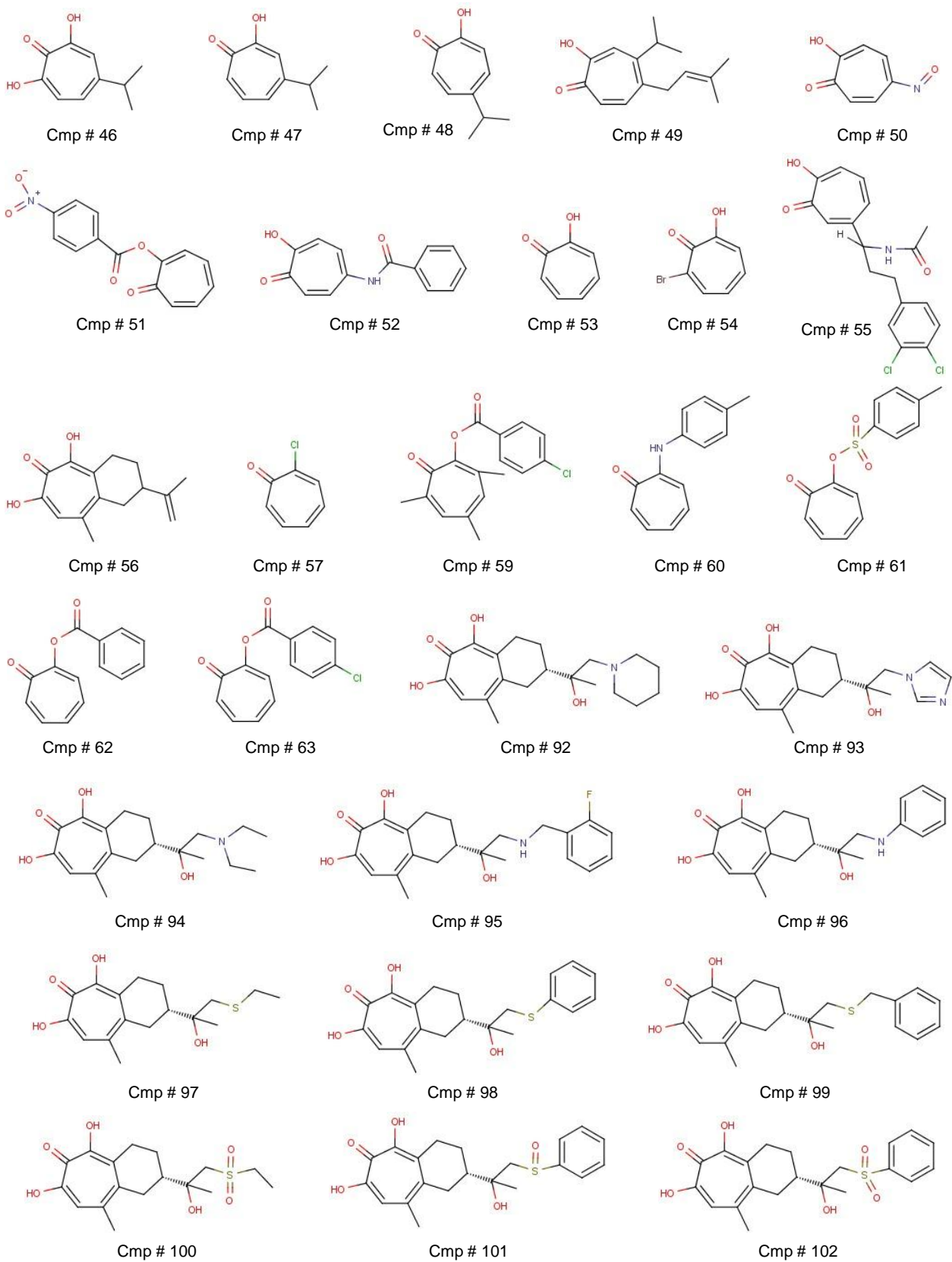
Figure 1S. Tropolones and related compounds employed in this study
