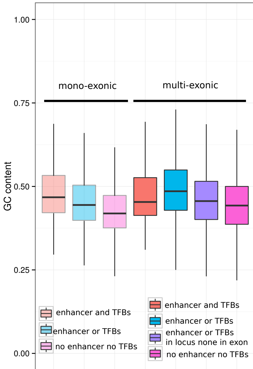
Supplementary Figure 2. GC content variation between lncRNAs exons depending upon gene model (mono-exonic, multi-exonic) and the presence of enhancers and TFBSs within the loci.
