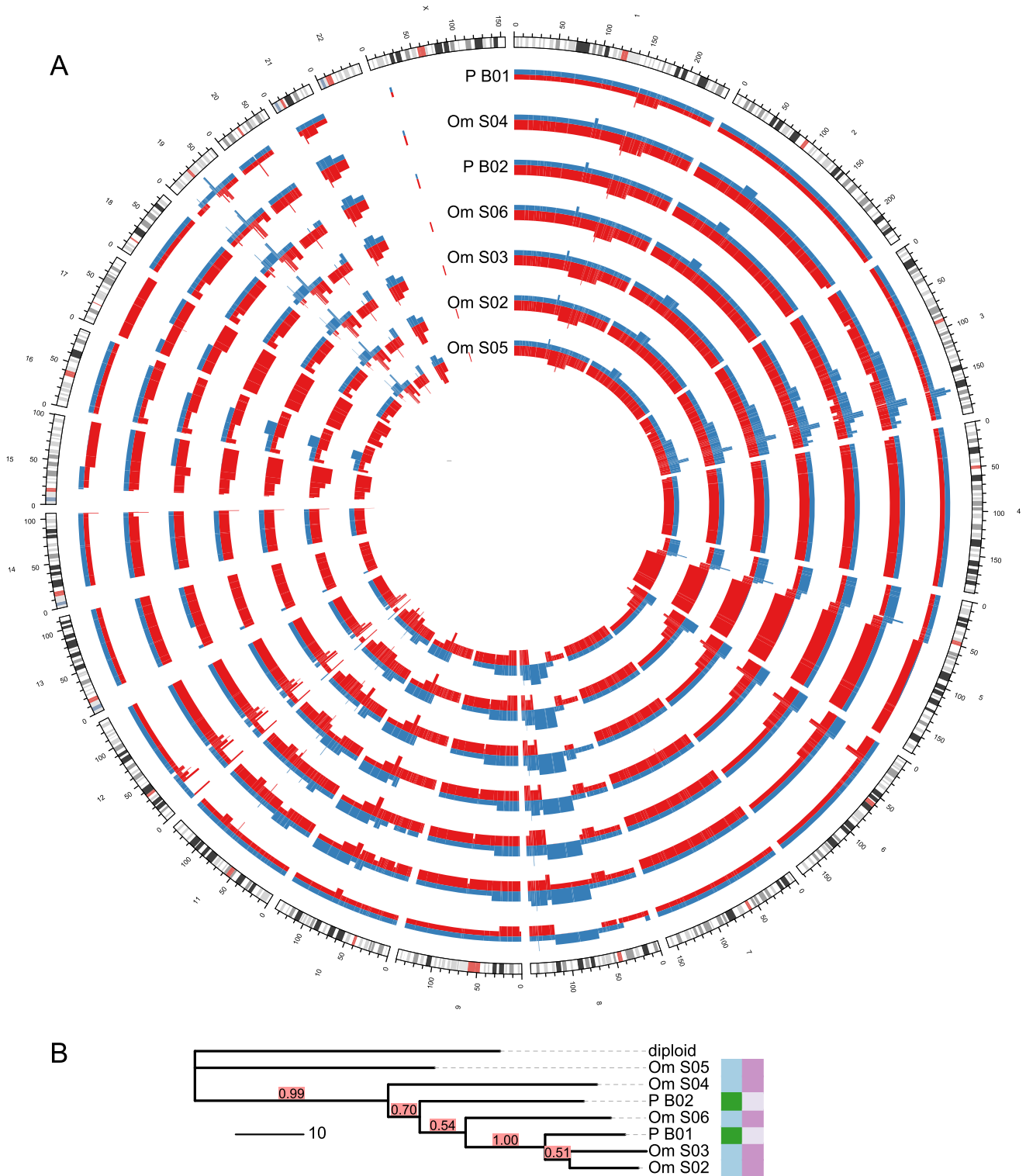
Figure 8: Copy-number (CN) profiles (A) and evolutionary tree (B) for case 7. Only selected CN profiles are shown and marked in bold in the evolutionary tree. Individual alleles are colored in red and blue. Confidence values for each split in the tree are given in red boxes. The color bars to the right of the tree indicate different sampling sites (left) and sampling times(right). Branch lengths are give in number of rearrangement events.
