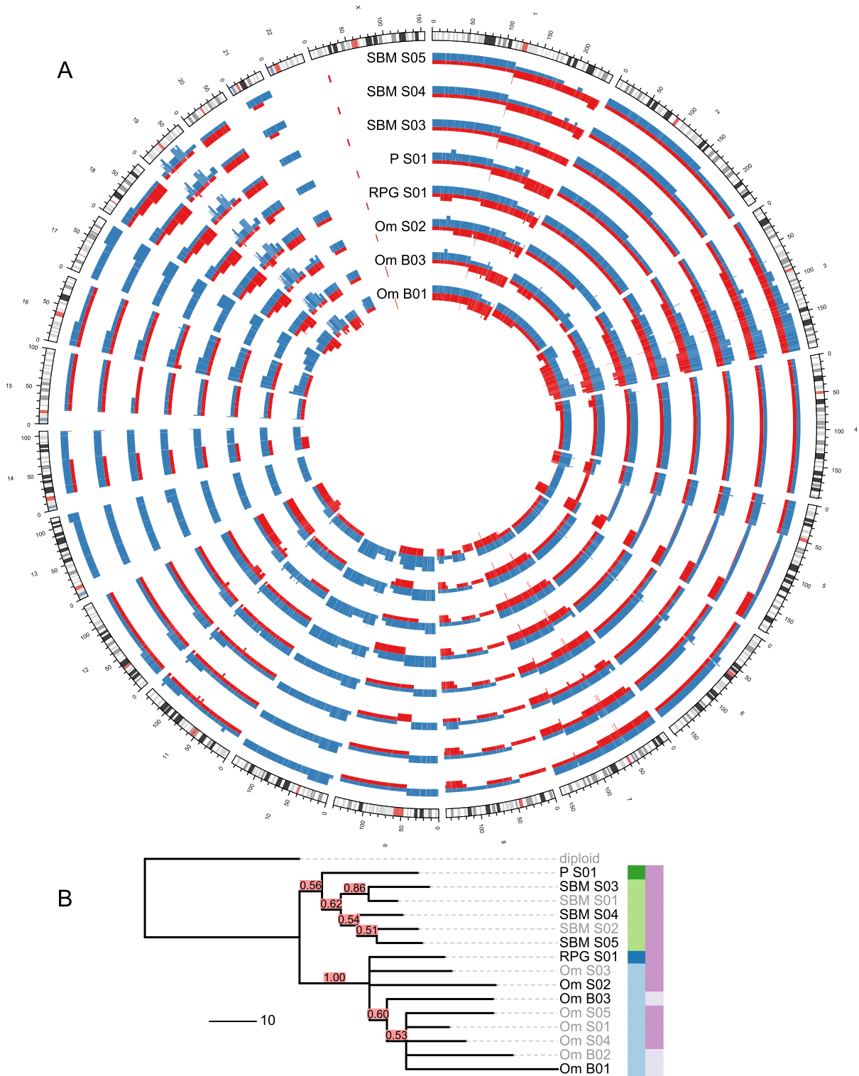
Figure 10: Copy-number (CN) profiles (A) and evolutionary tree (B) for case 9. Only selected CN profiles are shown and marked in bold in the evolutionary tree. Individual alleles are colored in red and blue. Confidence values for each split in the tree are given in red boxes. The color bars to the right of the tree indicate different sampling sites (left) and sampling times(right). Branch lengths are give in number of rearrangement events.
