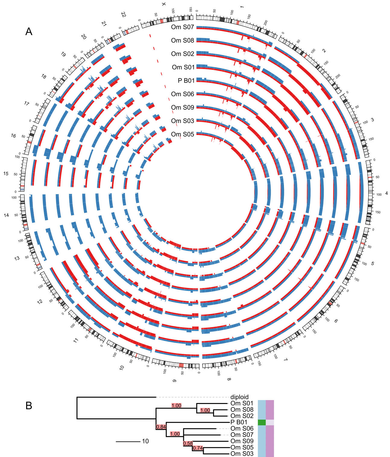
Figure 11: Copy-number (CN) profiles (A) and evolutionary tree (B) for case 10. Only selected CN profiles are shown and marked in bold in the evolutionary tree. Individual alleles are colored in red and blue. Confidence values for each split in the tree are given in red boxes. The color bars to the right of the tree indicate different sampling sites (left) and sampling times(right). Branch lengths are give in number of rearrangement events.
