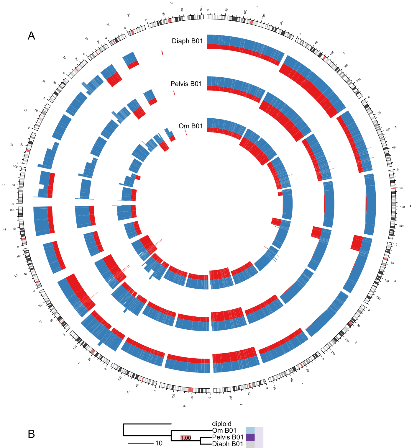
Figure 13: Copy-number (CN) profiles (A) and evolutionary tree (B) for case 13. Only selected CN profiles are shown and marked in bold in the evolutionary tree. Individual alleles are colored in red and blue. Confidence values for each split in the tree are given in red boxes. The color bars to the right of the tree indicate different sampling sites (left) and sampling times(right). Branch lengths are given in number of rearrangement events.
