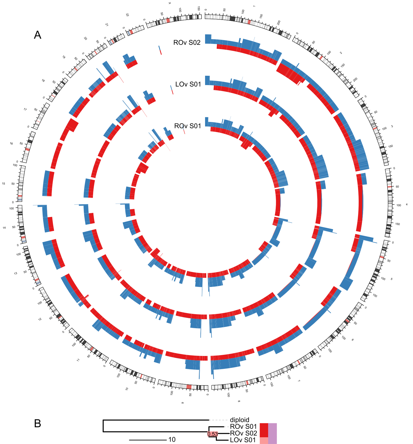
Figure 15: Copy-number (CN) profiles (A) and evolutionary tree (B) for case 15. Only selected CN profiles are shown and marked in bold in the evolutionary tree. Individual alleles are colored in red and blue. Confidence values for each split in the tree are given in red boxes. The color bars to the right of the tree indicate different sampling sites (left) and sampling times(right). Branch lengths are given in number of rearrangement events.
