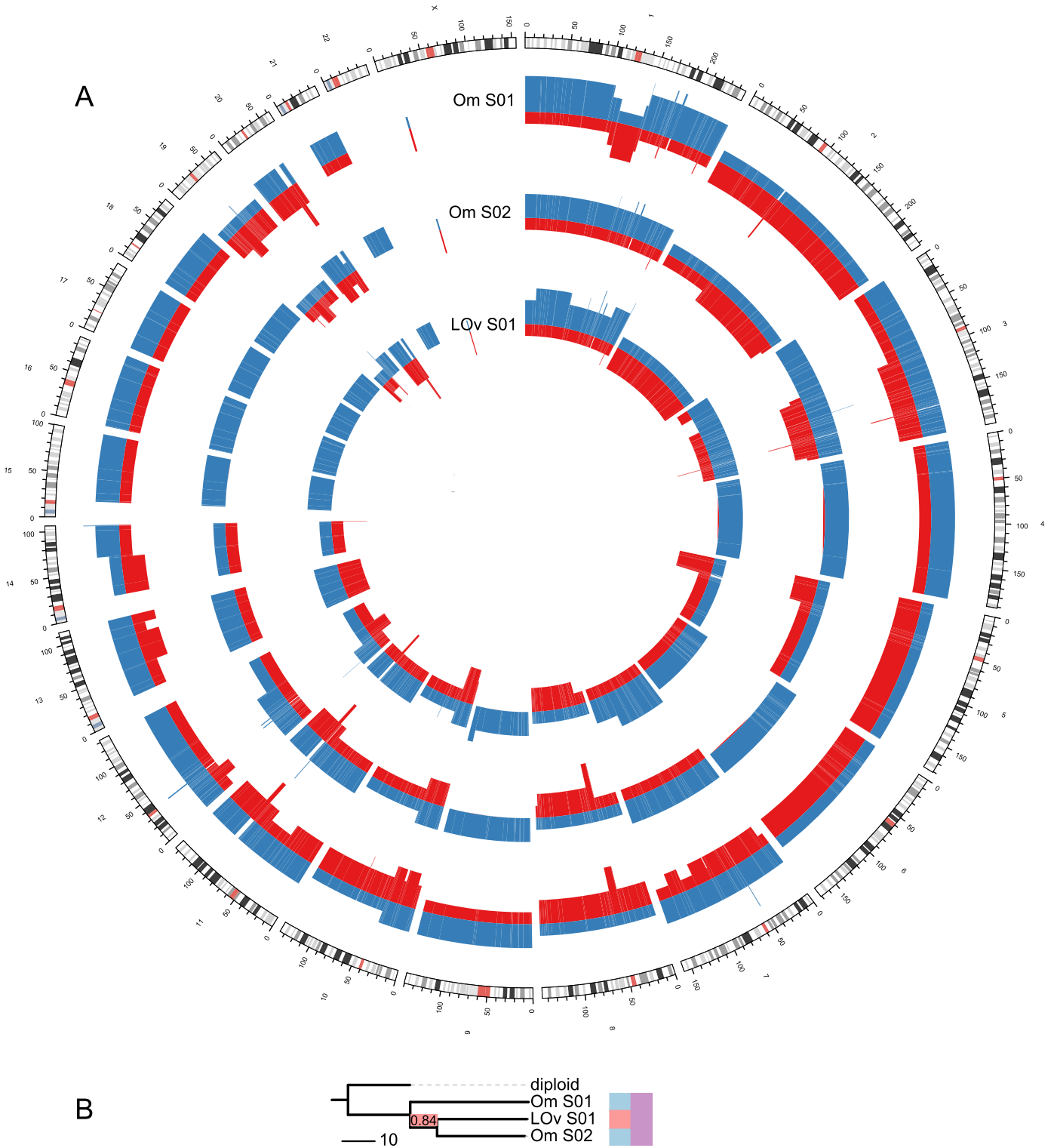
Figure 16: Copy-number (CN) profiles (A) and evolutionary tree (B) for case 17. Only selected CN profiles are shown and marked in bold in the evolutionary tree. Individual alleles are colored in red and blue. Confidence values for each split in the tree are given in red boxes. The color bars to the right of the tree indicate different sampling sites (left) and sampling times(right). Branch lengths are given in number of rearrangement events.
