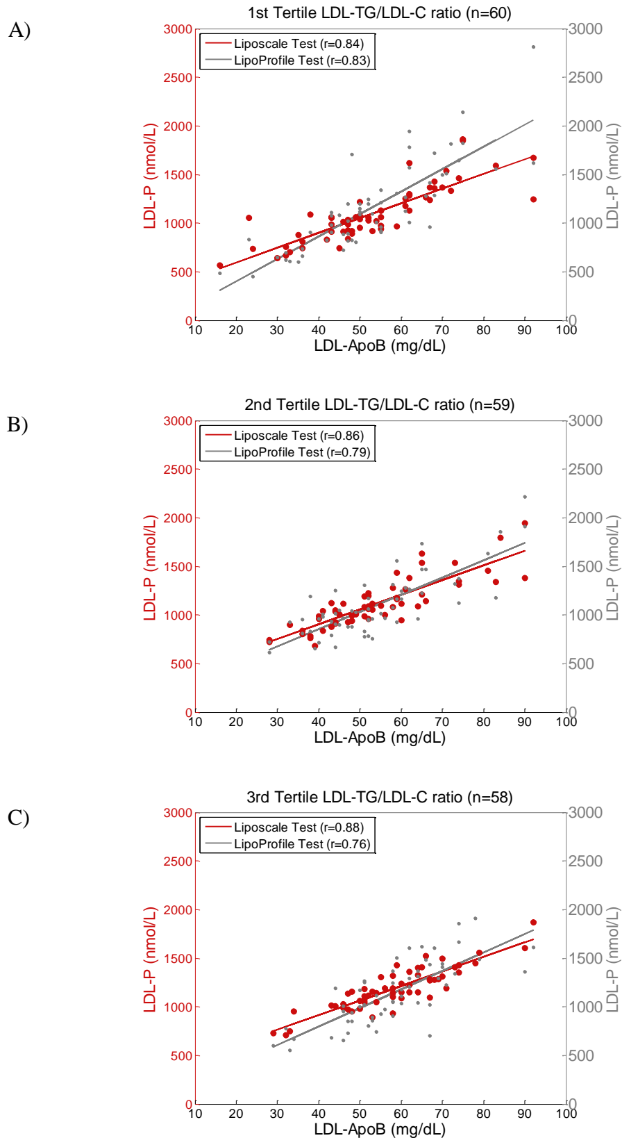
Figure 1. The plasma concentration of LDL-ApoB plotted against the plasma concentration of LDL-P across tertiles of the LDL-TG to LDL-C ratio: A) 1st tertile, B) 2nd tertile, and C) 3rd tertile.
