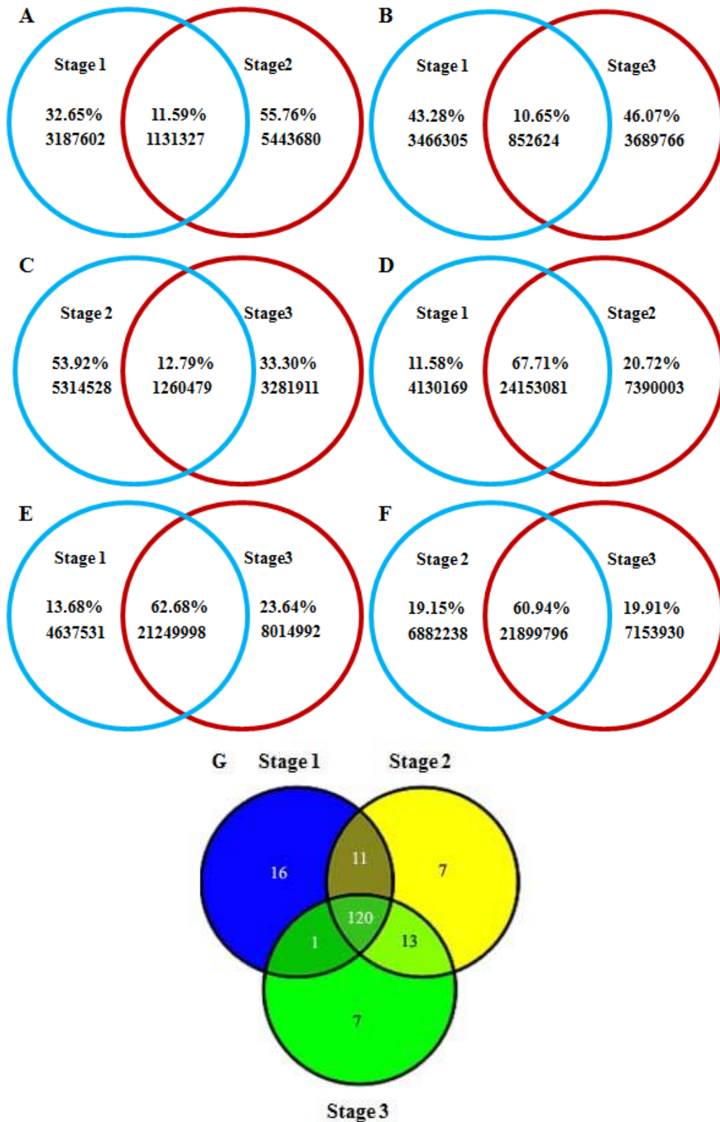
Additional file 3. Venn diagrams for analysis of Small RNAs. (A-F) Summary of common and specific unique (A, B and C) sRNAs and total ( D, E and F) sRNAs between different libraries. (G) Known miRNAs among different libraries.
