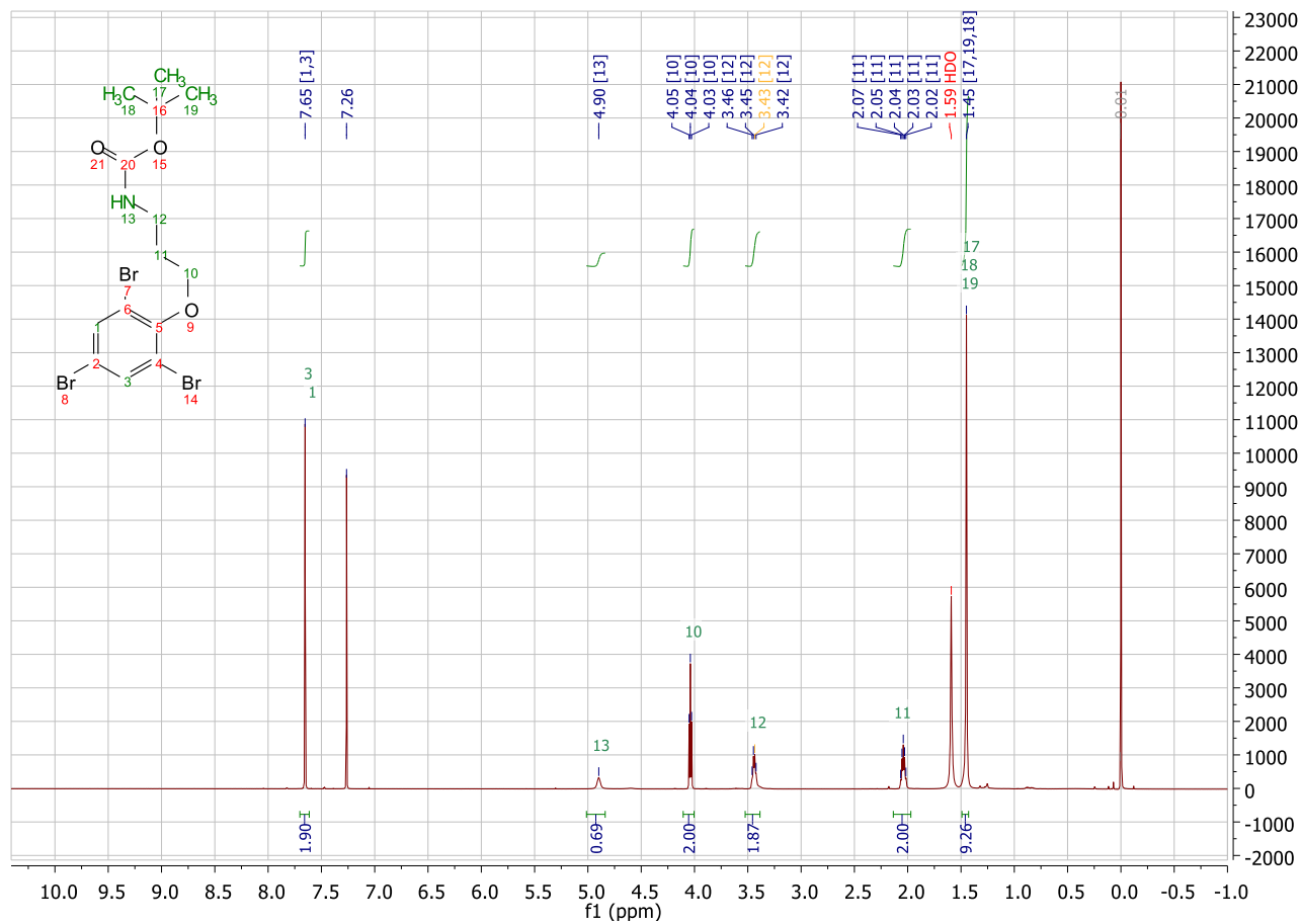
Figure S3. ^1\text{H} NMR of 5
