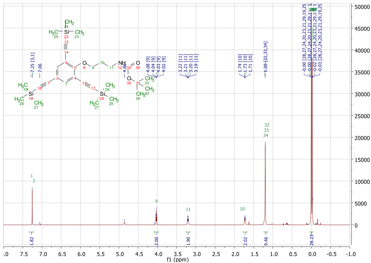
Figure S5: 1 H NMR of 6
