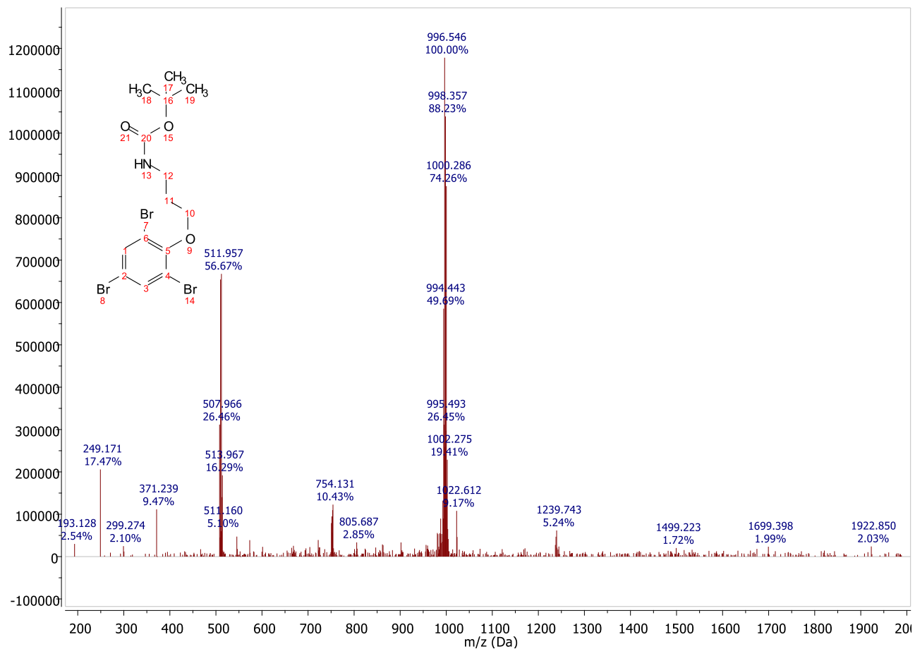
Figure S12. MS (ESI-positive) of 5
