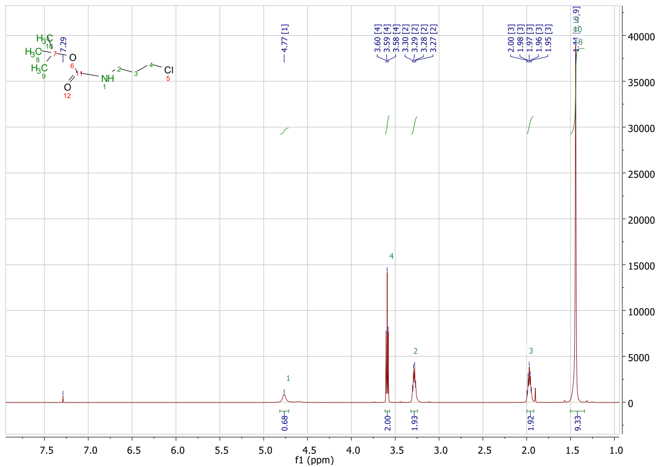
Figure S1. ^1\text{H} NMR of 4
