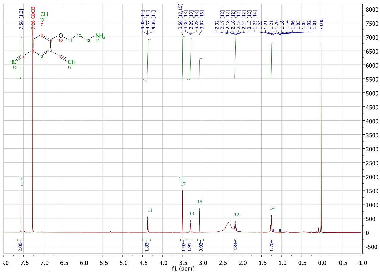
Figure S9. 1 H NMR of 8
