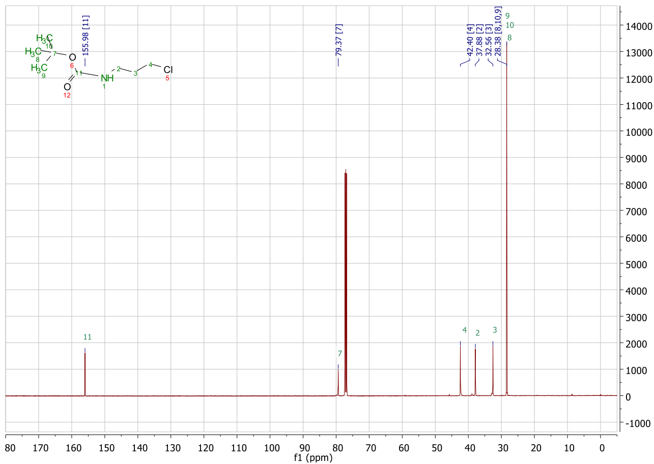
Figure S2. ^{13}\text{C} NMR of 4
