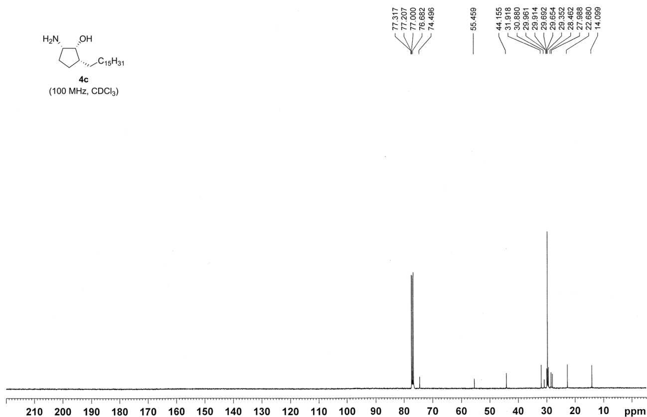
Figure S30. 13 C NMR spectrum of 4c .
