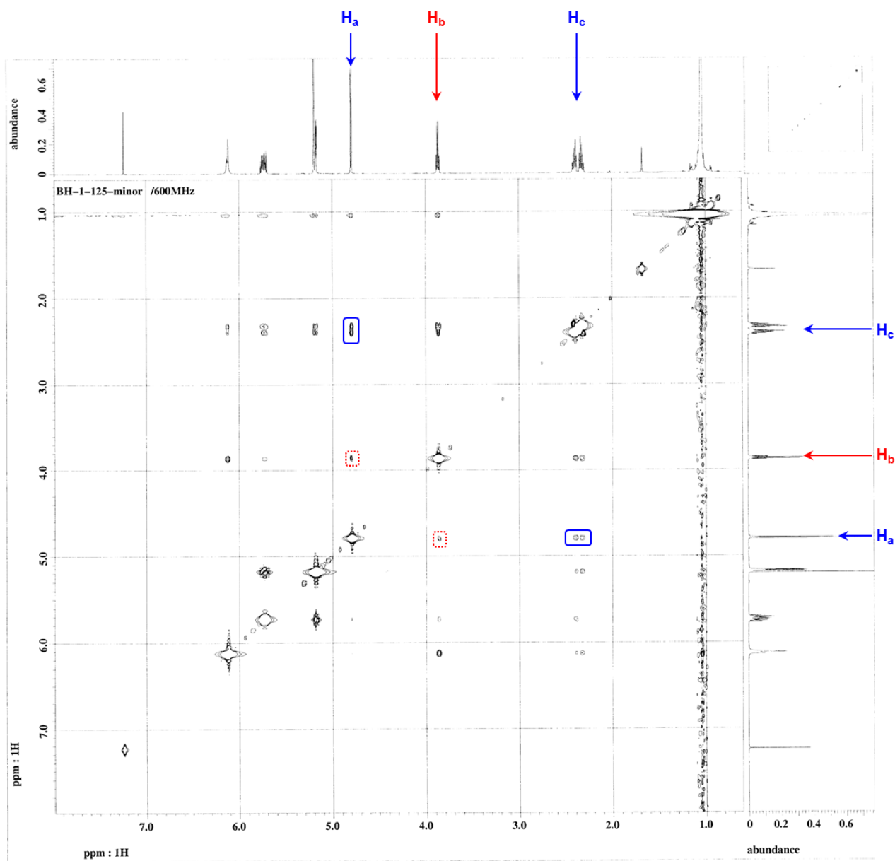
Figure S10. 2D NOESY spectrum of 10b .
