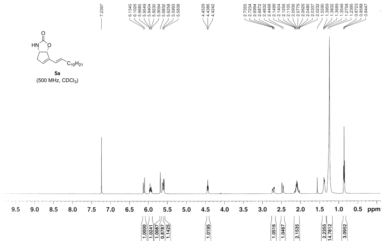
Figure S13. 1 H NMR spectrum of 5a .
