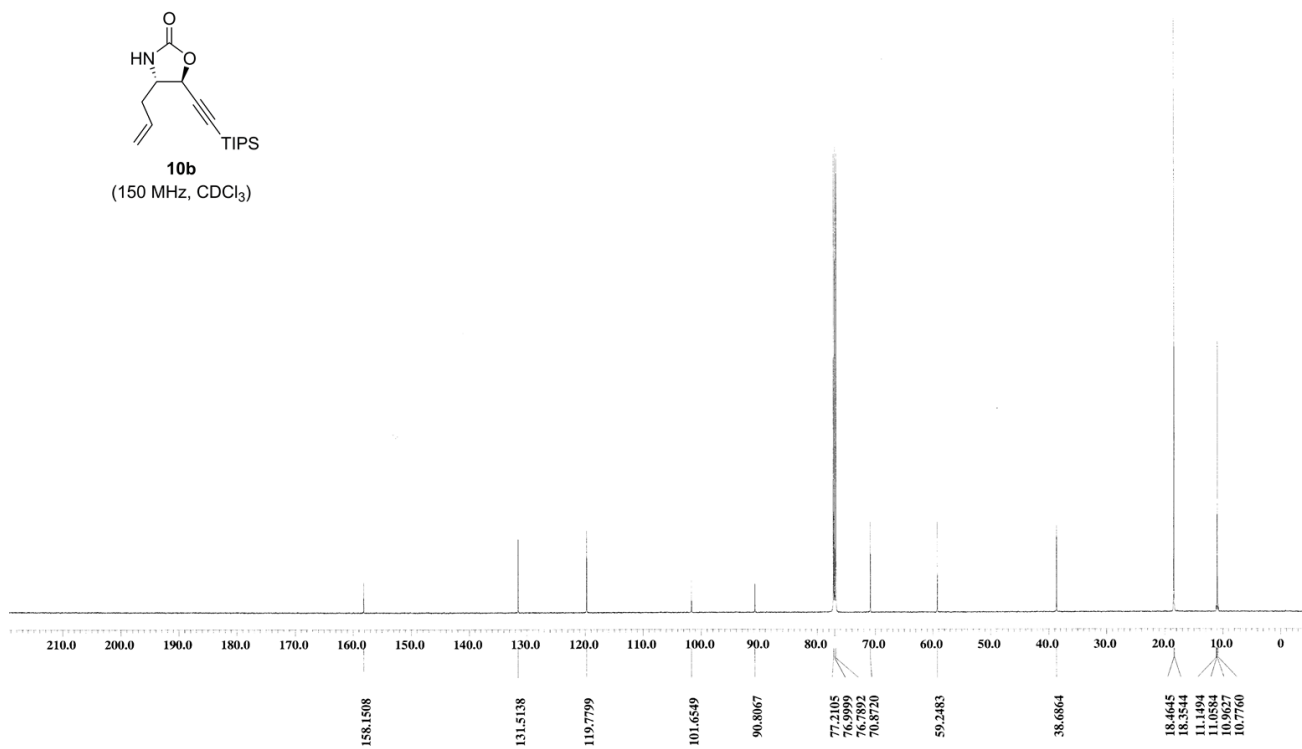
Figure S9. 13 C NMR spectrum of 10b .
