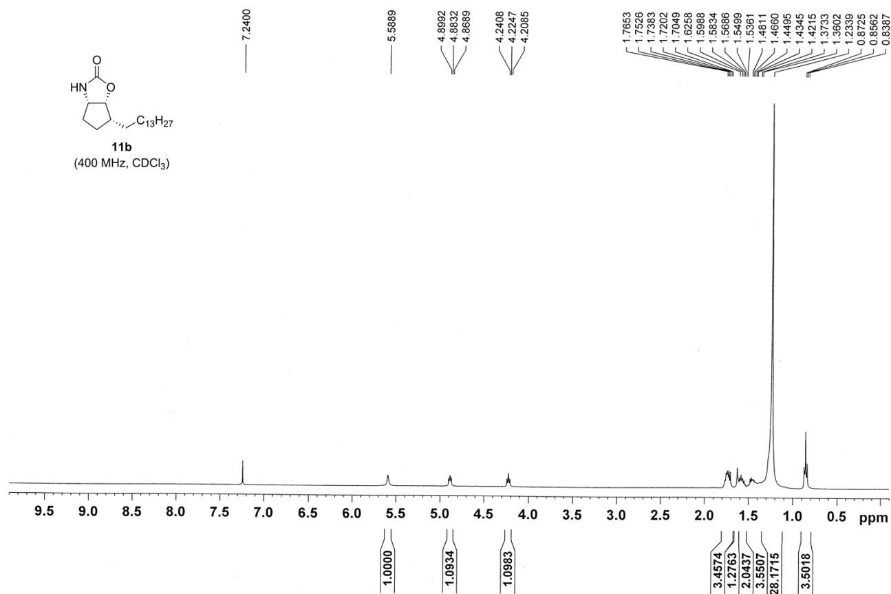
Figure S21. 1 H NMR spectrum of 11b .
