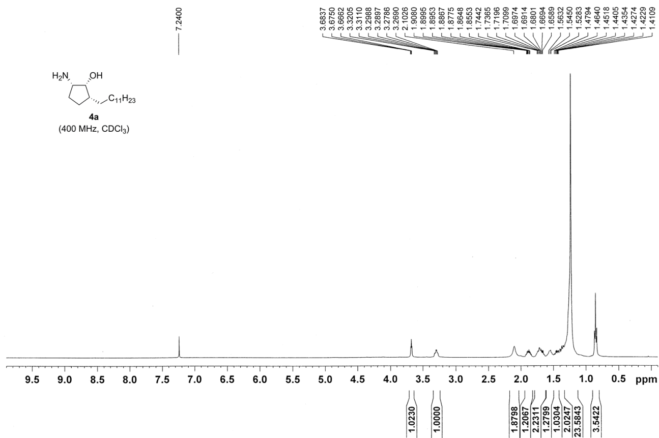
Figure S25. 1 H NMR spectrum of 4a .
