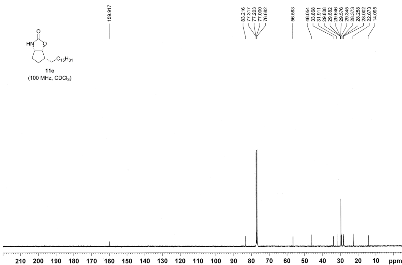
Figure S24. 13 C NMR spectrum of 11c .
