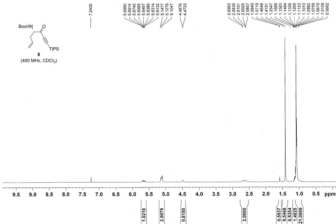
Figure S1. 1 H NMR spectrum of 8 .
