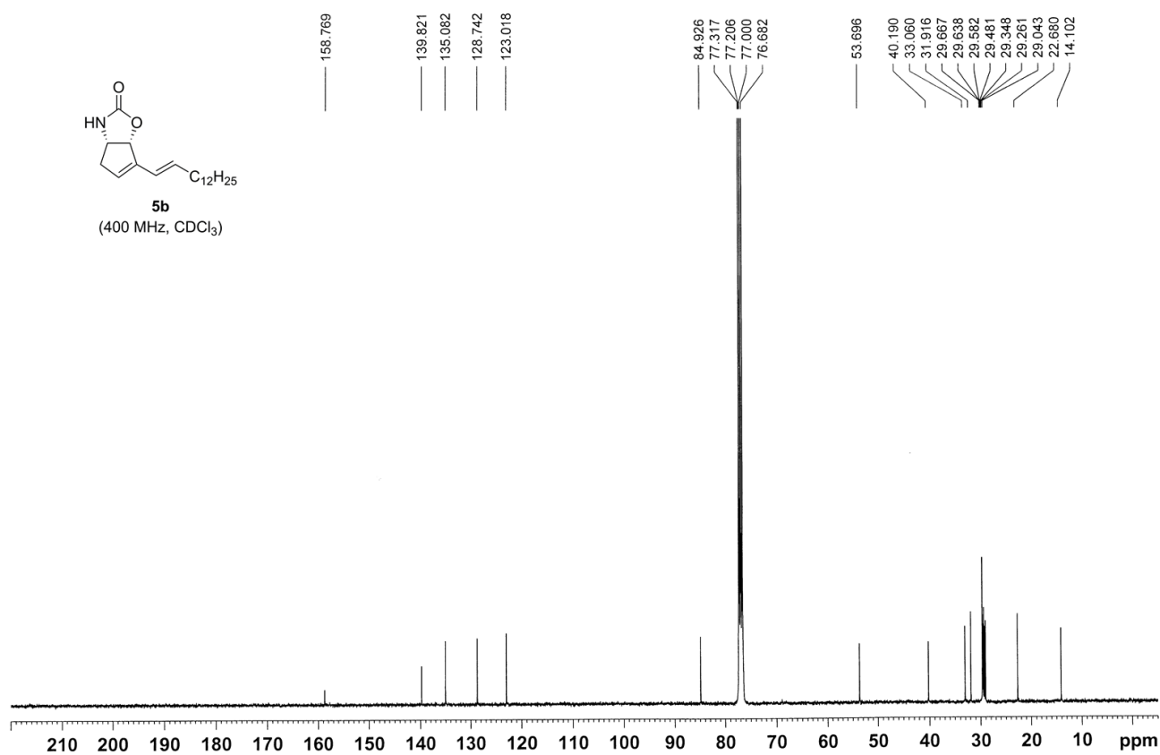
Figure S16. 13 C NMR spectrum of 5b .
