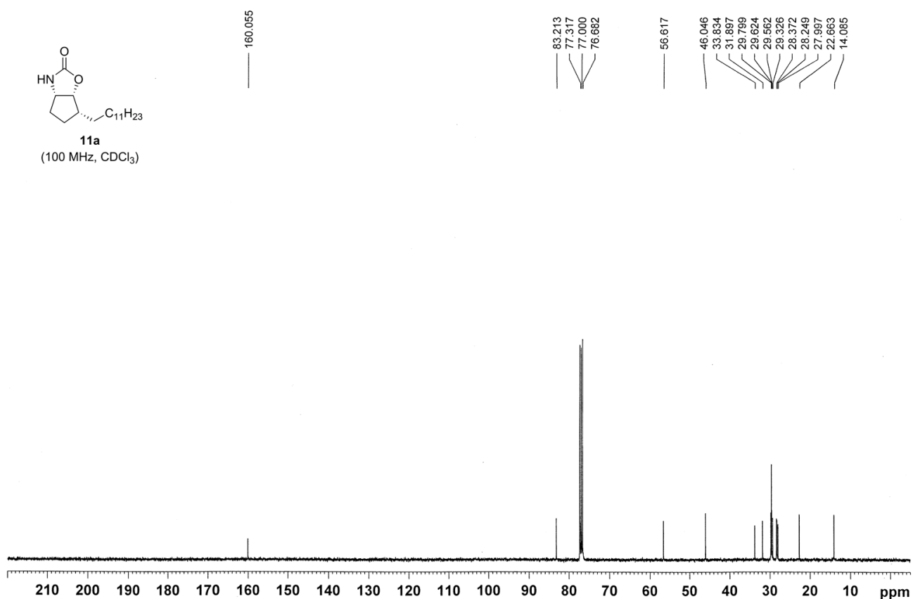
Figure S20. 13 C NMR spectrum of 11a .
