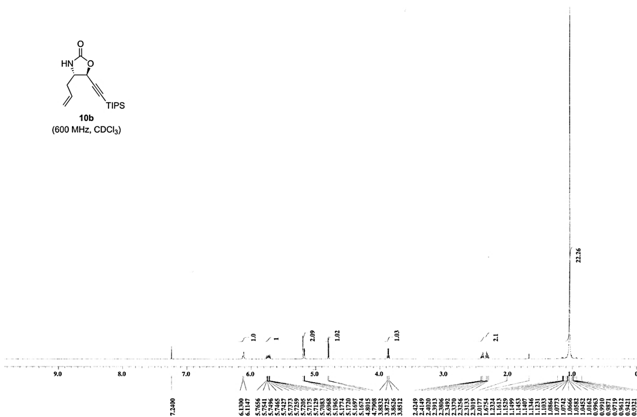
Figure S8. 1 H NMR spectrum of 10b .
