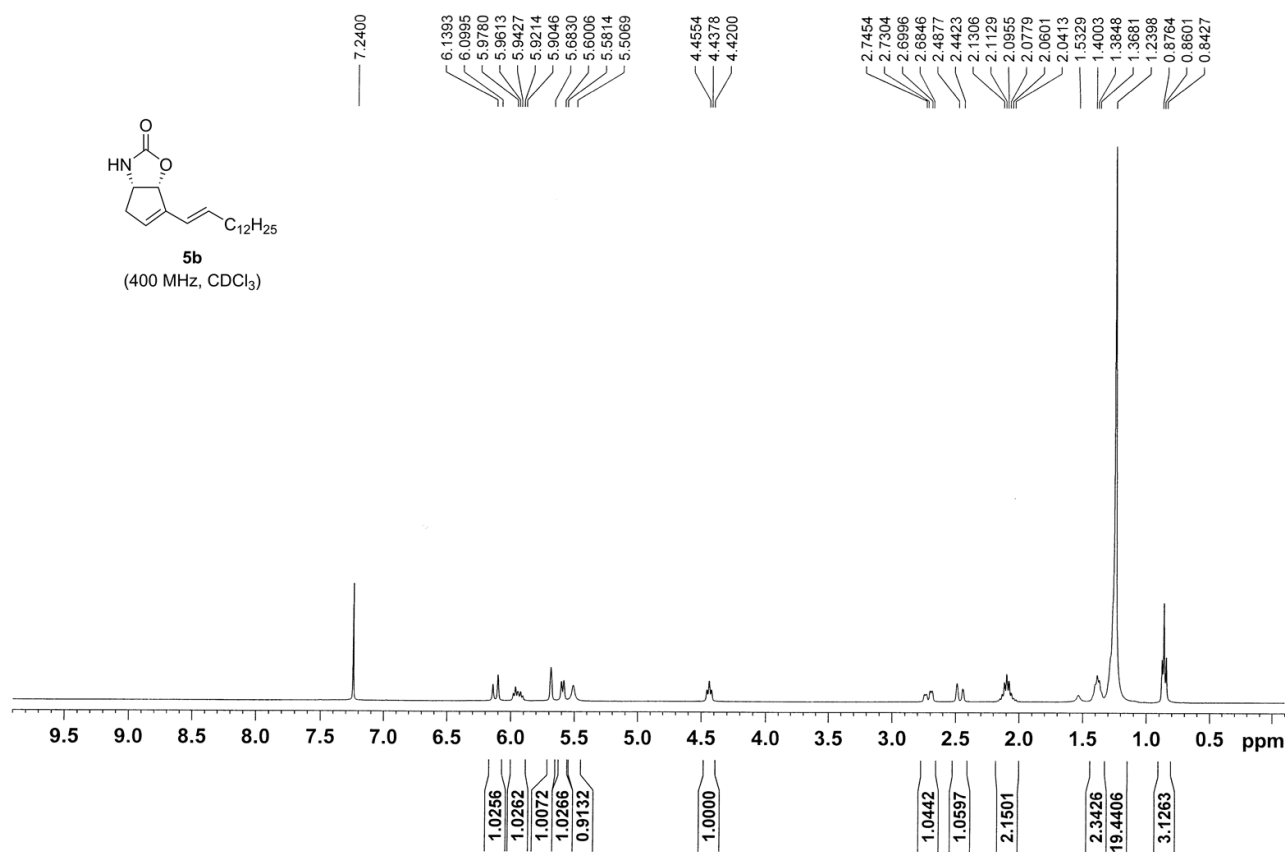
Figure S15. 1 H NMR spectrum of 5b .
