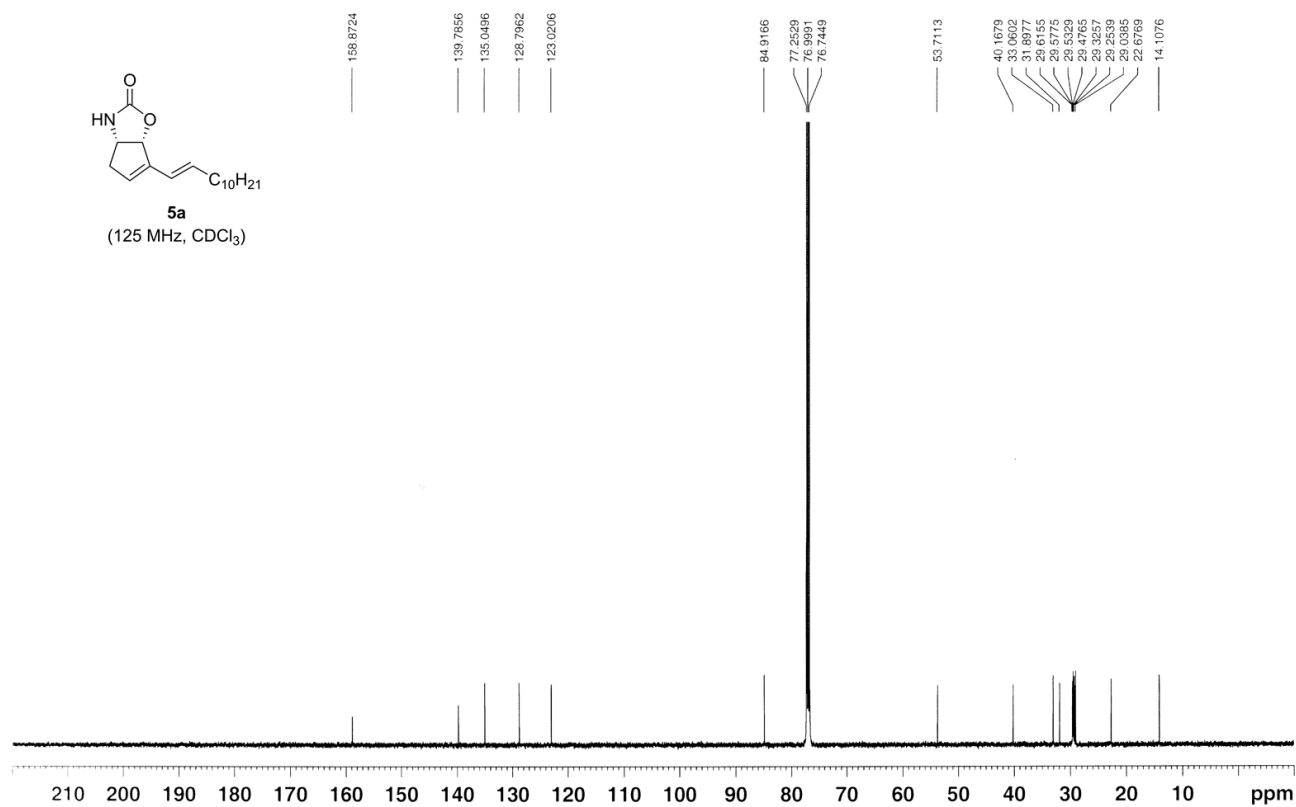
Figure S14. 13 C NMR spectrum of 5a .
