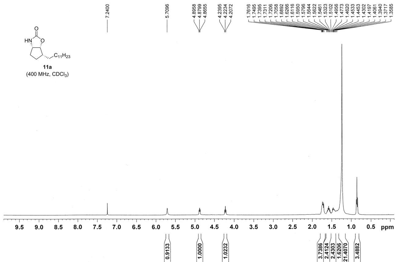
Figure S19. 1 H NMR spectrum of 11a .
