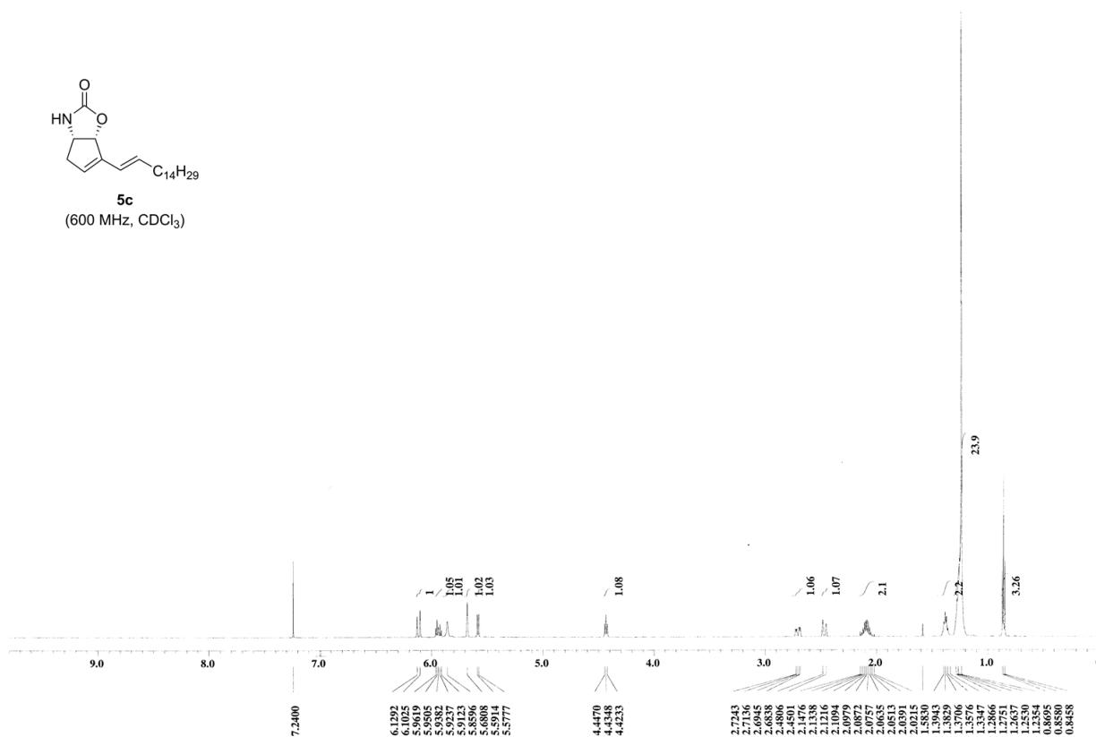
Figure S17. 1 H NMR spectrum of 5c .
