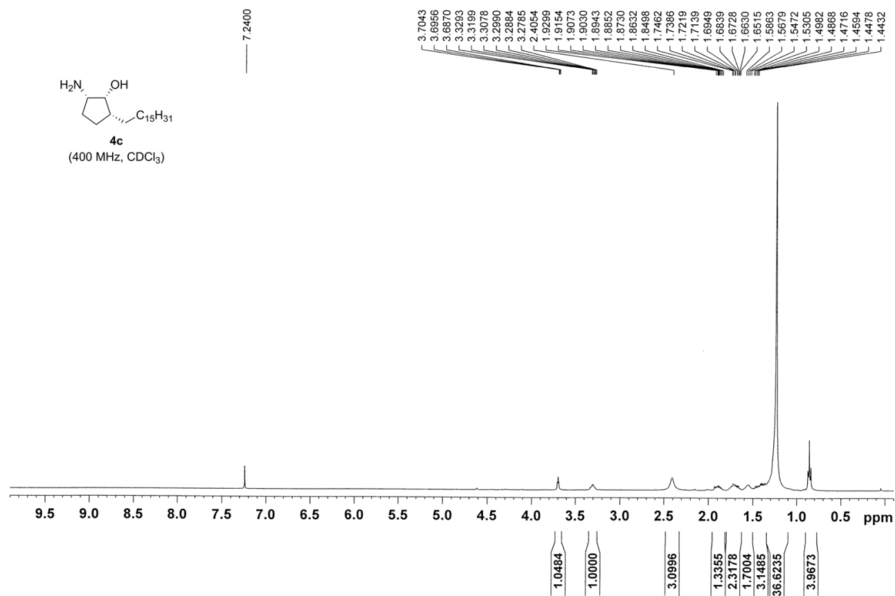
Figure S29. 1 H NMR spectrum of 4c .
