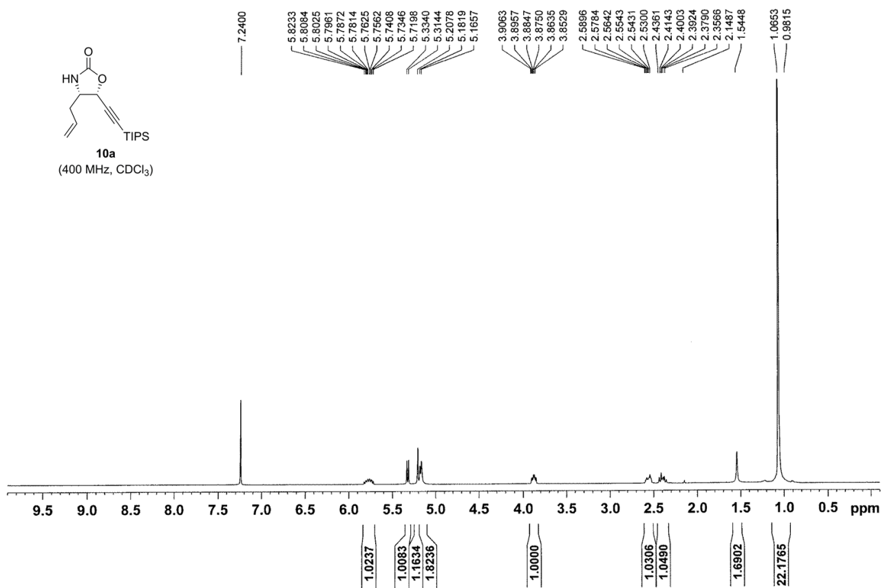
Figure S5. 1 H NMR spectrum of 10a .
