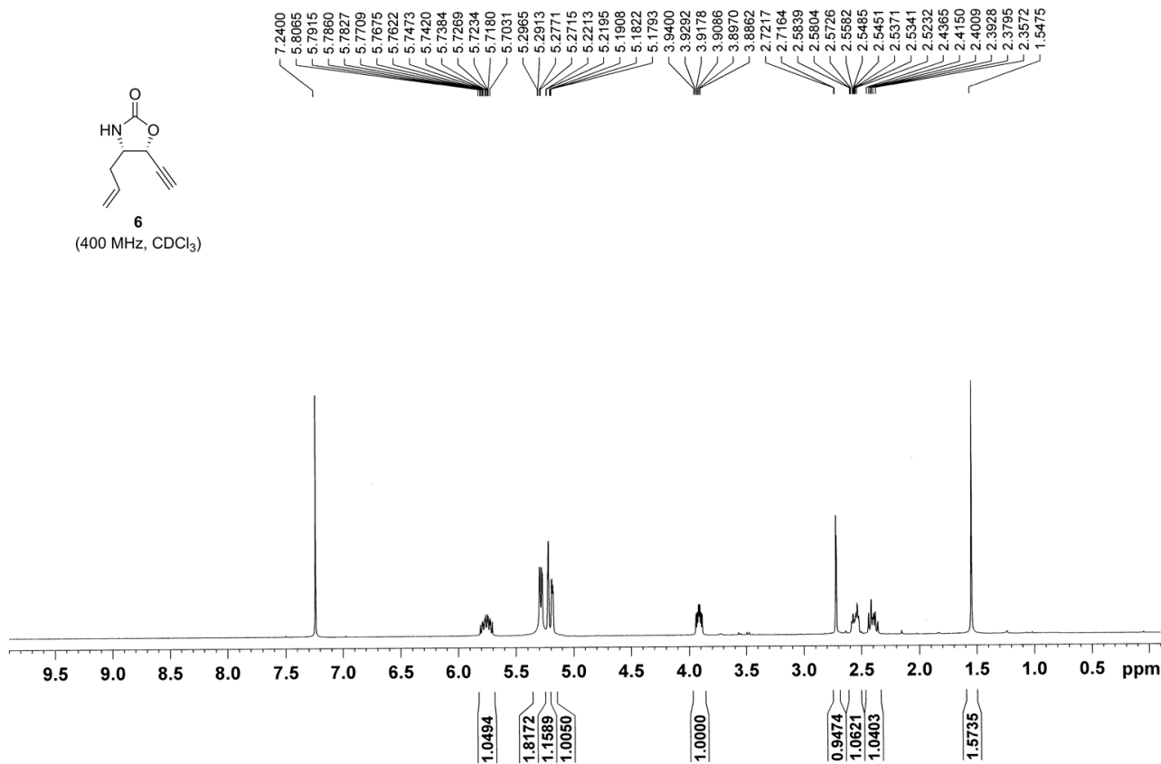
Figure S11. 1 H NMR spectrum of 6 .
