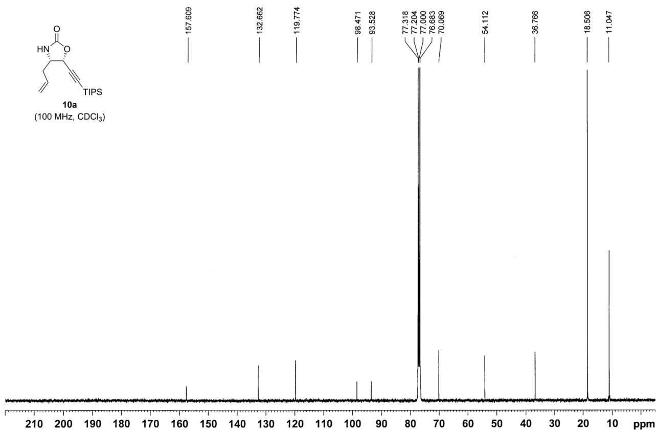
Figure S6. 13 C NMR spectrum of 10a .
