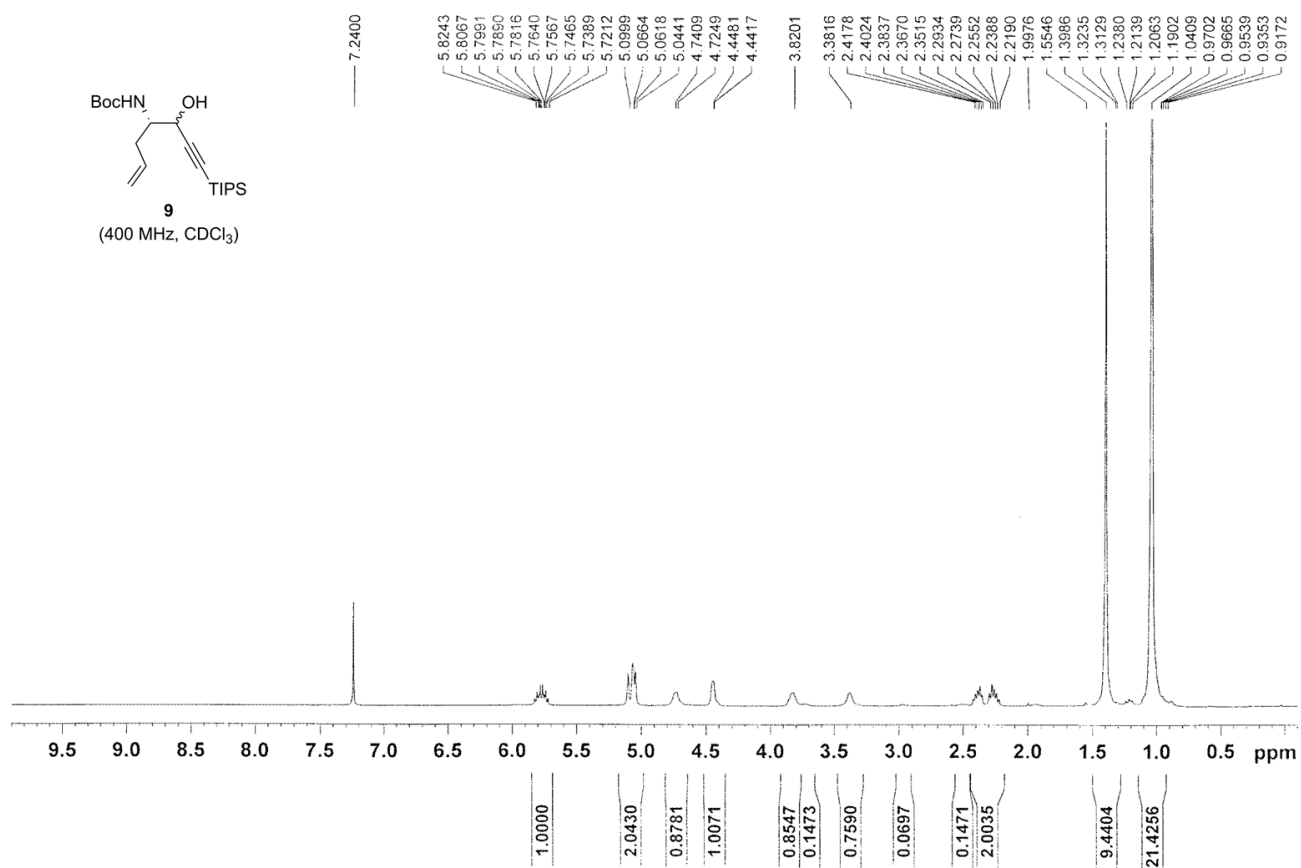
Figure S3. 1 H NMR spectrum of 9 .
