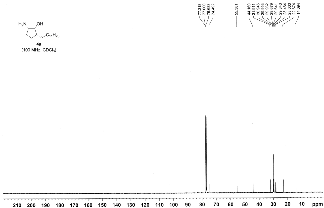
Figure S26. 13 C NMR spectrum of 4a .
