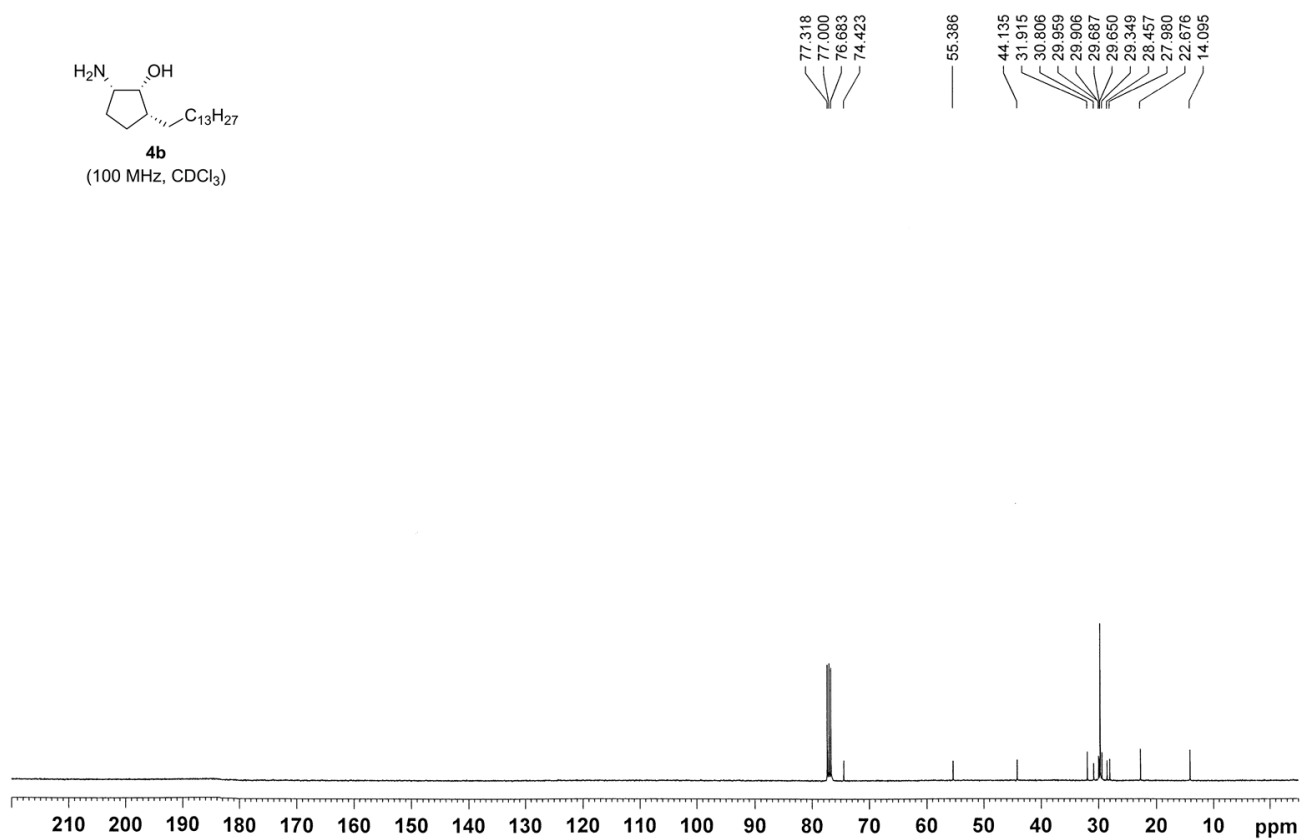
Figure S28. ^{13}\text{C} NMR spectrum of 4b .
