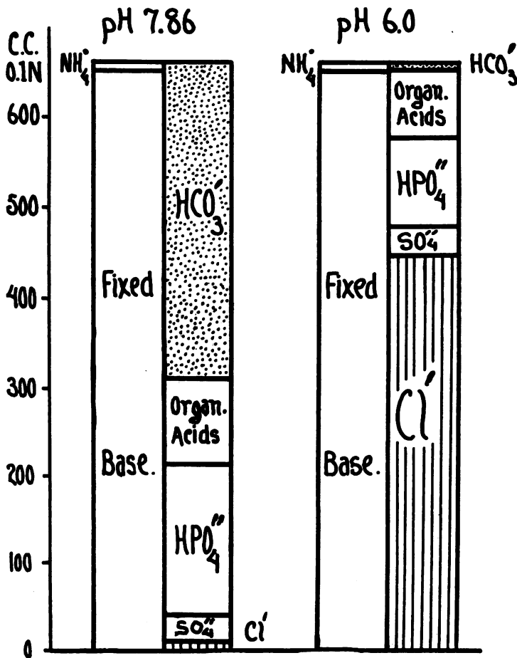
FIG. 5. ILLUSTRATING THE EXTENT OF CONSERVATION OF Cl' OBTAINED BY PRODUCTION OF SPECIMEN NO. 4 (TABLE 7) AT pH 7.86 INSTEAD OF AT THE USUAL REACTION OF URINE, pH 6.0
