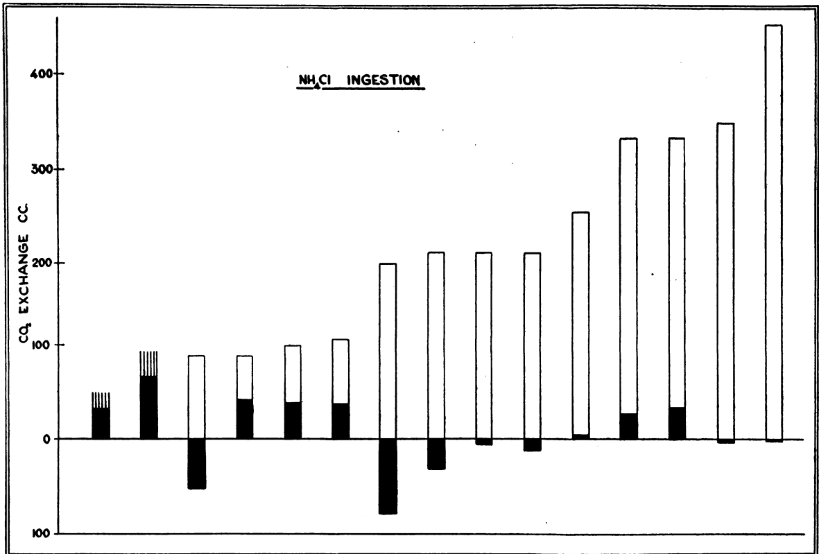
FIG. 3. EXCHANGES OF \text{CO}_2 FOLLOWING INGESTION OF \text{NH}_4\text{Cl}
