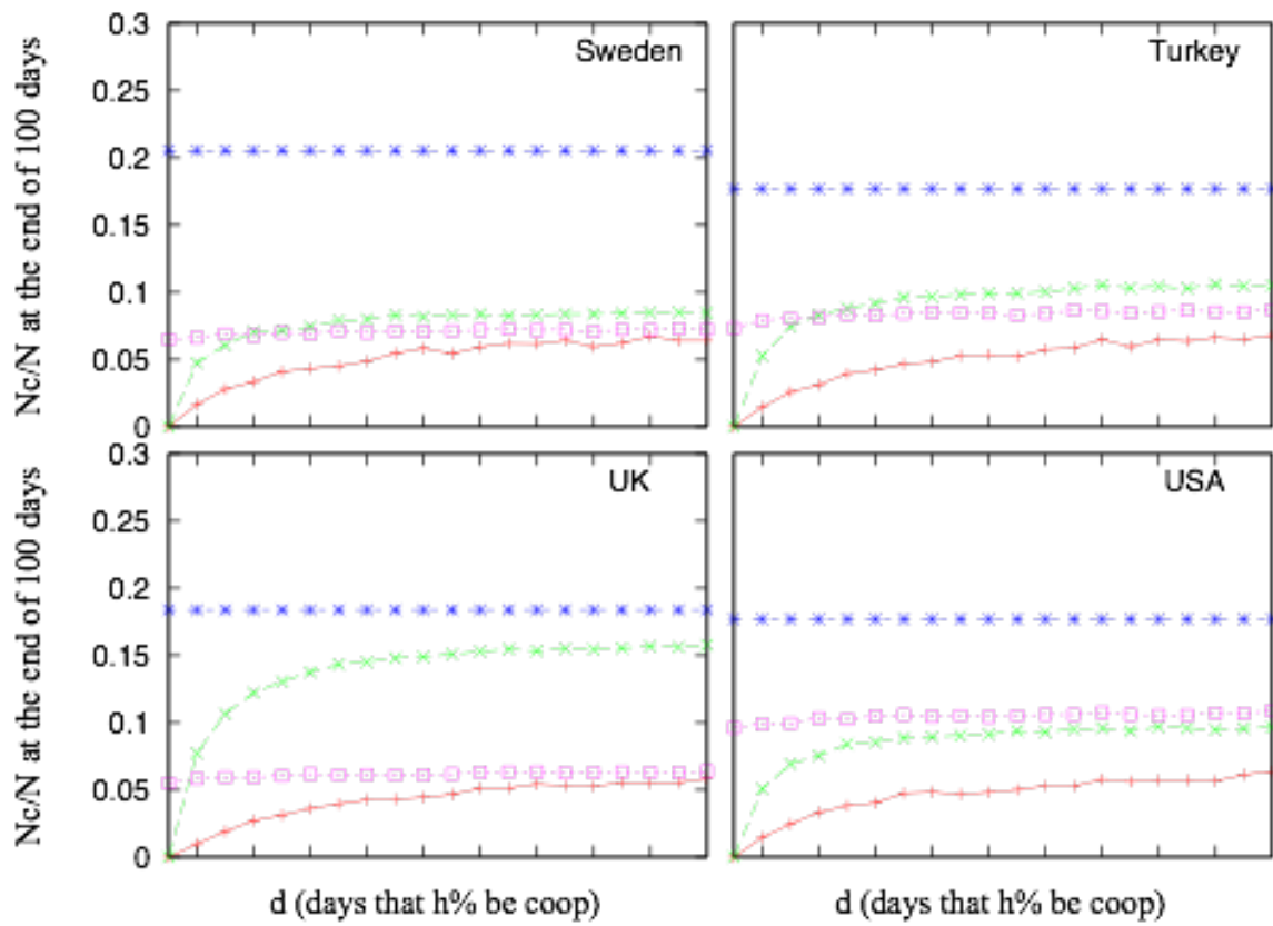
Figure S4. The learning curve for non-cooperative personalities. We fix h = 0.50 and simulate the model for various d to see how the outcome of cooperation will improve for non-cooperative personalities. The results are shown for personality distribution of Sweden, Turkey, UK and USA.
