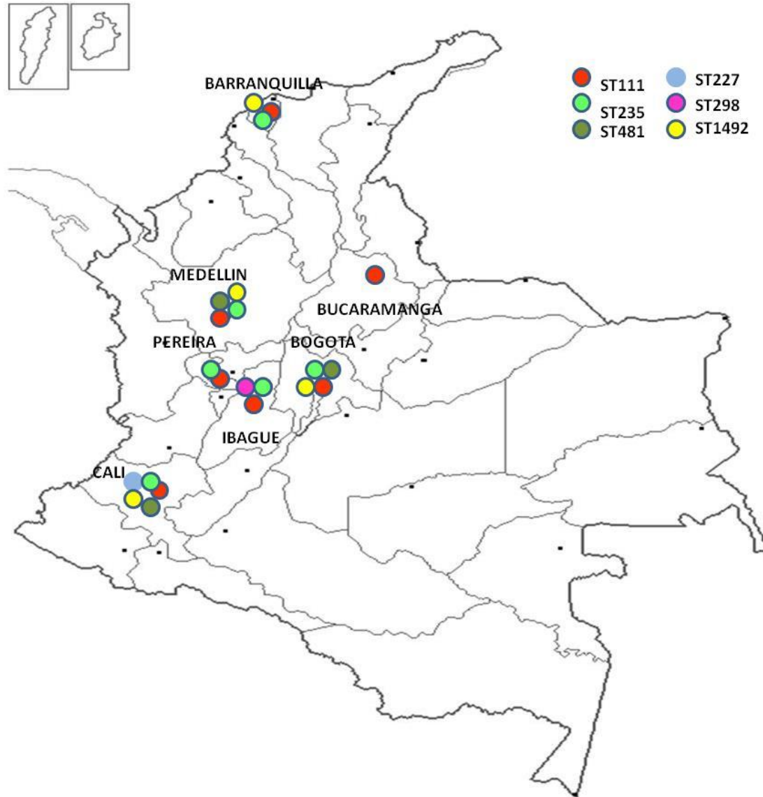
Figure S1: Sequence types (STs) of Pseudomonas aeruginosa found in seven Colombian cities.
