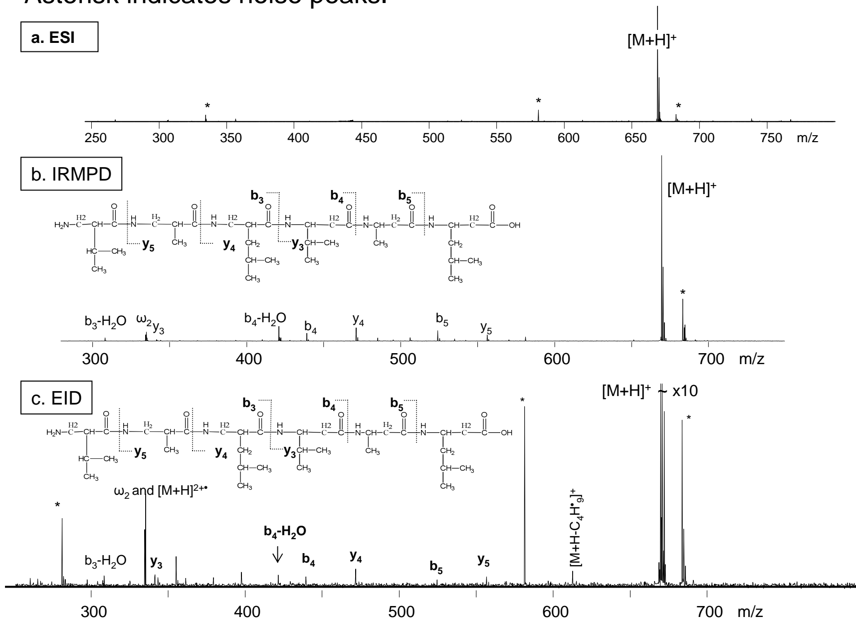
Figure S2. Q 06 beta peptide \beta_2 V_{\beta_2} A_{\beta_2} L_{\beta_3} V_{\beta_3} A_{\beta_3} L : a. ESI, b. IRMPD, c. EID. Asterisk indicates noise peaks.
