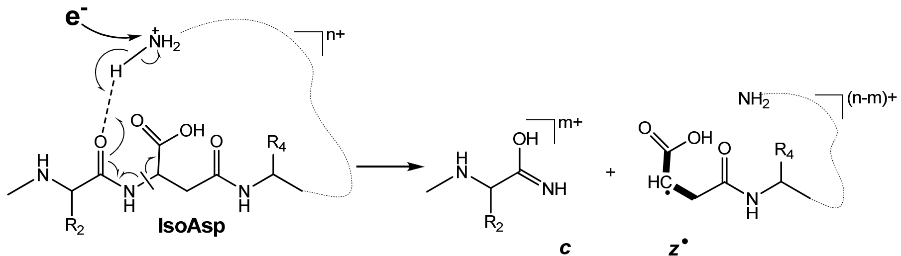
Figure S1. ECD of isoaspartic acid
