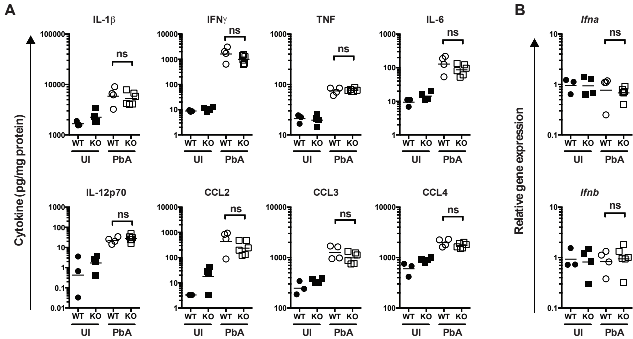
Figure S3. Effect of Irgm3 deficiency on spleen cytokine levels on day 3 p.i. WT or Irgm3 -/- (KO) mice were infected with PbA on day 0. On day 3 p.i., groups of uninfected (UI) and PbA-infected mice were euthanized and cytokine protein ( A ) or mRNA ( B ) were quantified. ( A ) Levels of the indicated cytokines/chemokines were measured by cytometric bead array and normalized to total protein concentration within the homogenate. ( B ) Relative levels of the indicated cytokine genes were determined by RT-qPCR. Data are from a single experiment. Statistical significance was determined using ANOVA with Tukey's post-test. Symbols represent individual mice, and horizontal bars are the geometric mean of groups. n.s., p>0.05.
